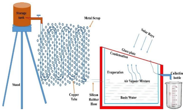
Figure 2. SSSS with metal scrap Heat Enhancers
