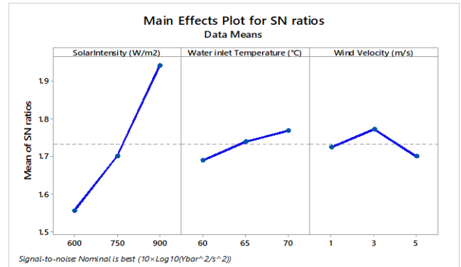
Figure 4. Main Effects Plot for Means of S/N ratios Taguchi Optimization Process
