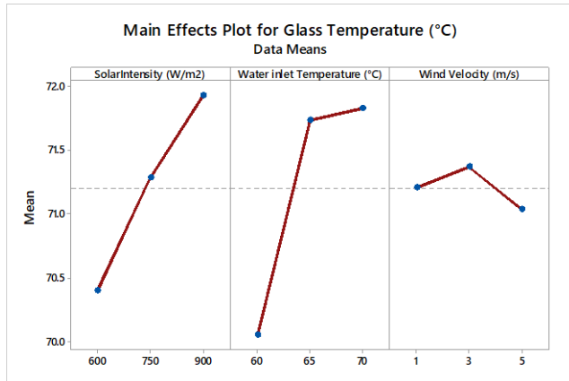
Figure 6. Main Effects plot for Tg in Taguchi Analysis.
