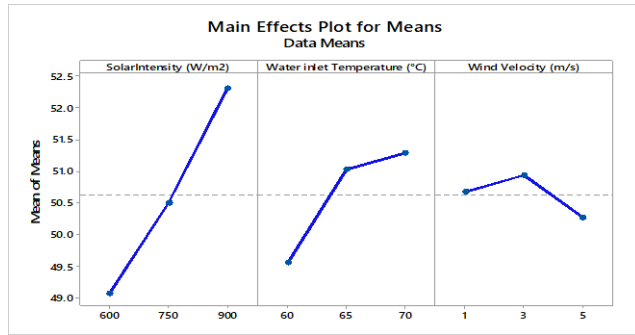
Figure 3. Main Effects Plot for Means in Taguchi Optimization Process
