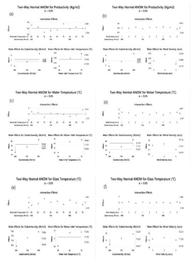
Figure 11. Two way Normal ANOM for Output Responses
