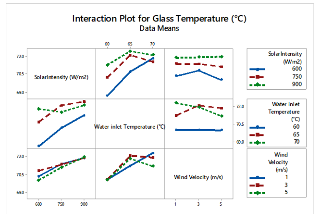
Figure 9. Interaction Plot for Tg in Taguchi Analysis
