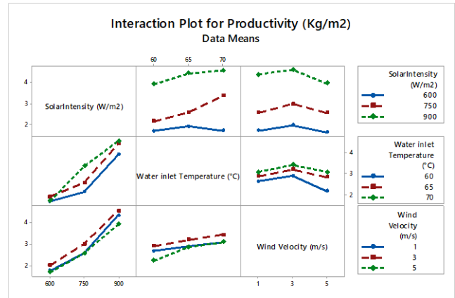
Figure 8. Interaction Plot for P in Taguchi Analysis
