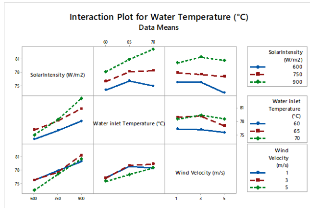
Figure 10. Interaction Plot for T_w in Taguchi Analysis
