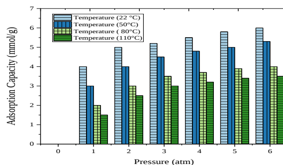
Figure 6. CO 2 Adsorption Performance Trends Across Varying Conditions
