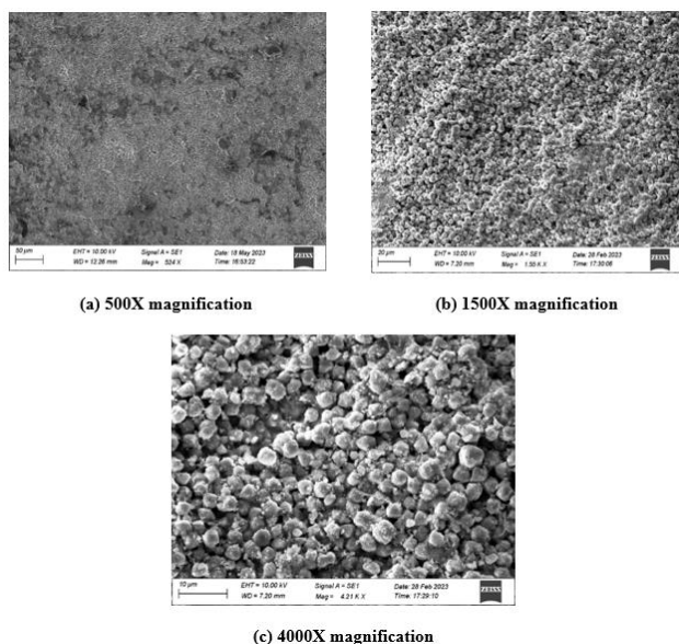
Figure 10. SEM images of Zeolite 13x after CO 2 capture
