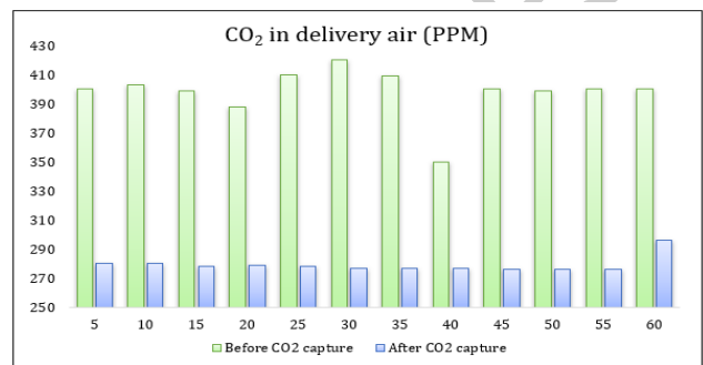
Figure 4. Amount of CO 2 present in delivery air (ppm) before and after CO 2 capture
