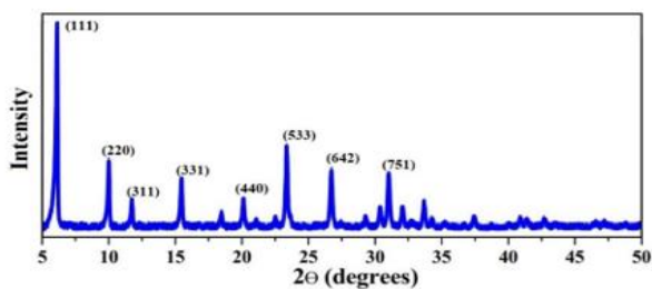
Figure 12. XRD analysis of Zeolite
