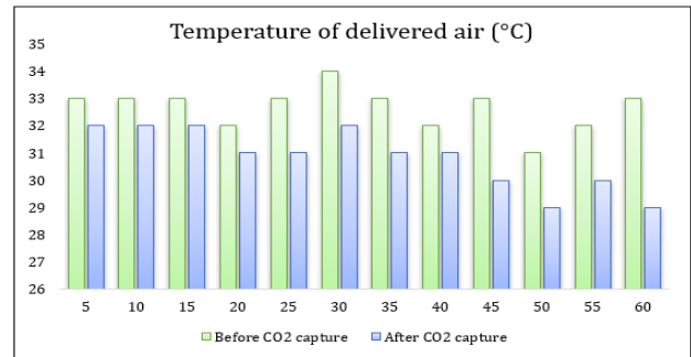
Figure 3. Temperature comparison of delivery air before and after CO 2 capture
