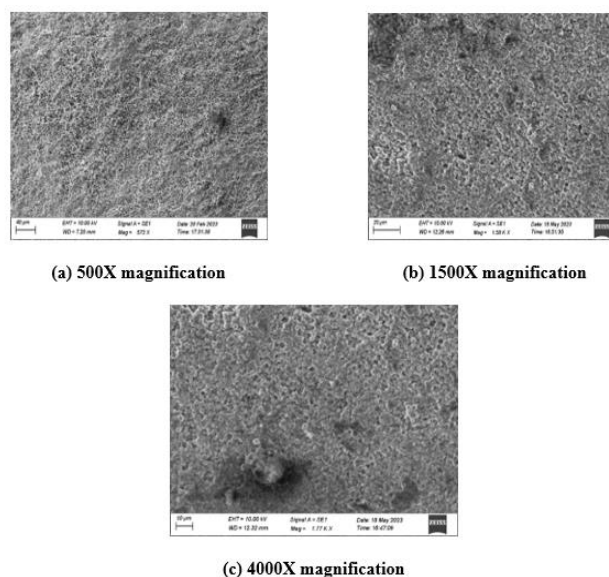
Figure 11. SEM images of Zeolite 13x after CO 2 capture
