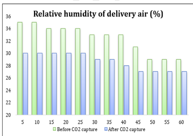
Figure 5. Relative humidity of delivery air (%) before and after CO 2 capture
