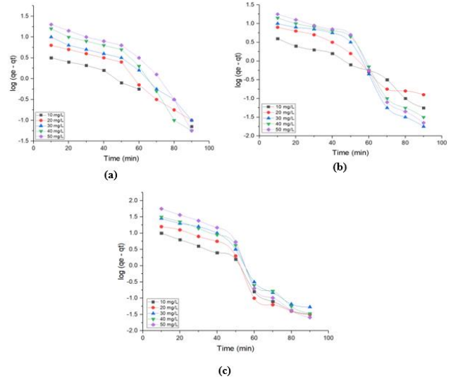
Figure 11. Pseudo-first-order kinetic plots for (a) CR, (b) CV, and (c) MB dyes adsorption
