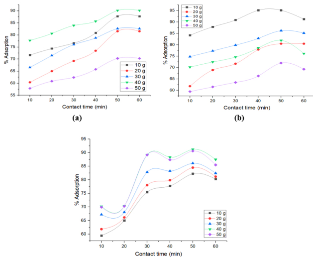
Figure 6 Effect of reaction time (min) variation on adsorption efficiency for (a) Pb, (b) Cd, and (c) Cu ions
