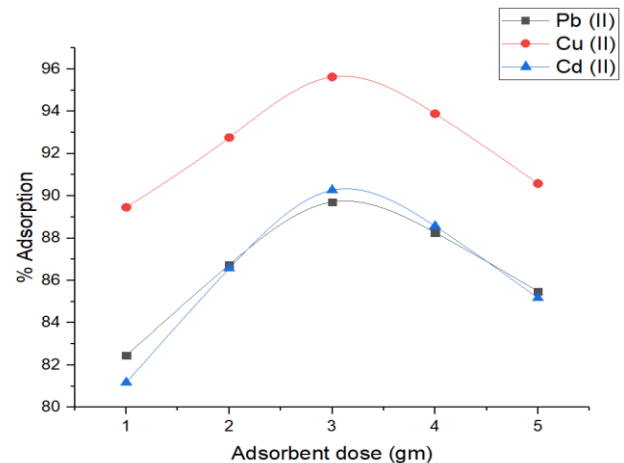
Figure 4 Effect of adsorbent dose variation on adsorption efficiency
