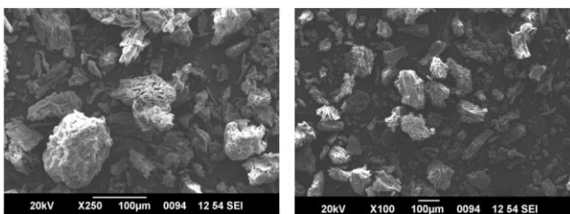
Figure 2. (a) Raw and (b) metal ions adsorbed PJRP biosorbent SEM image
