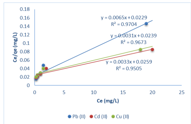
Figure 8 Langmuir isotherm plot for heavy metal adsorption using Prosopis juliflora roots
