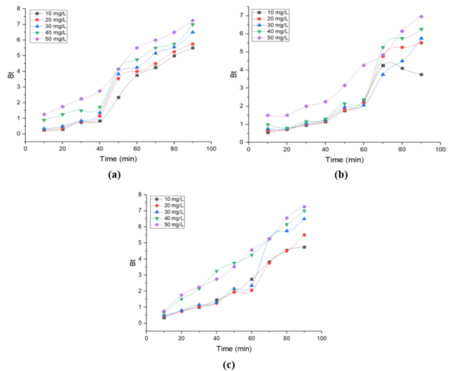
Figure 13 Boyd kinetic plots for (a) Pb, (b) Cd, and (c) Cu metal ion adsorption
