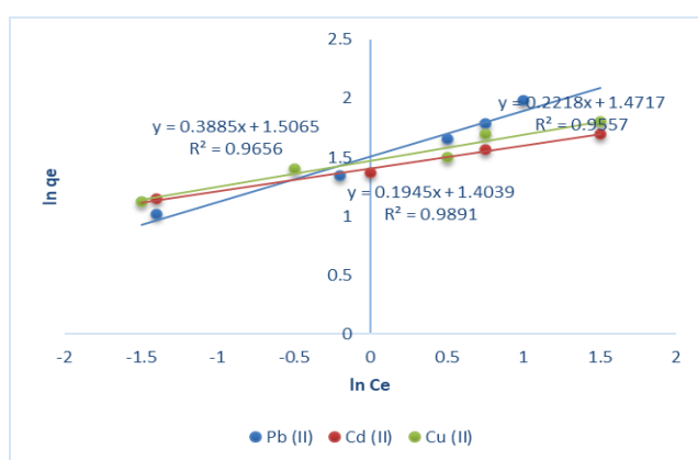
Figure 9 Freundlich isotherm plot for heavy metal adsorption using Prosopis juliflora roots
