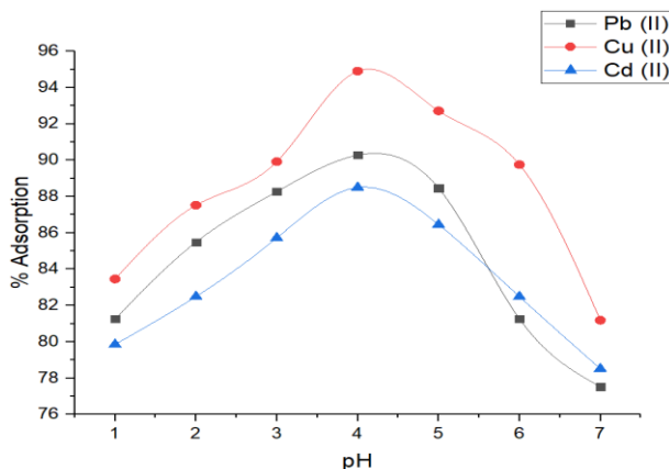
Figure 3 Effect of pH variation on adsorption efficiency
