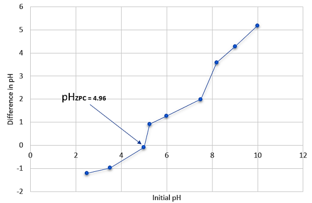
Figure 7 pH_{zpc} of the batch adsorption studies
