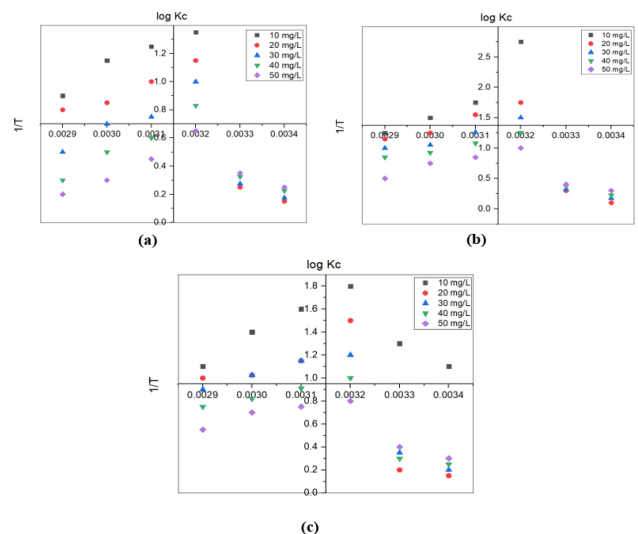
Figure 14 Thermodynamic plots for (a) Pb, (b) Cu, and (c) Cd metal ions using PJRP
