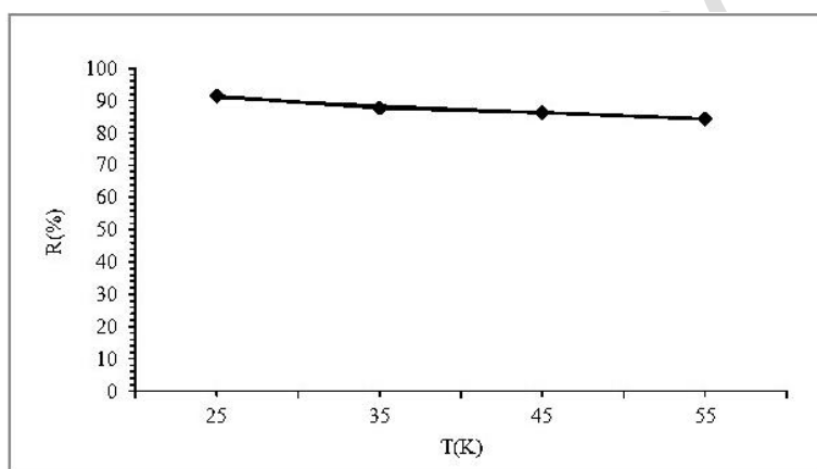
Figure 6: Effect of temperature on adsorption capacity of MB onto activated peanut shells.
