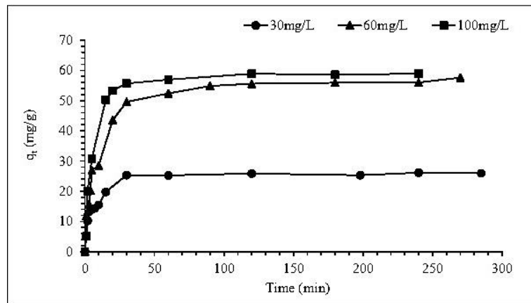
Figure 5: Effect of contact time and MB concentration on adsorption capacity onto NaOH-activated peanut shells. pH= 6.6, dose of adsorbent=1g/L, T=24± 2°C.
