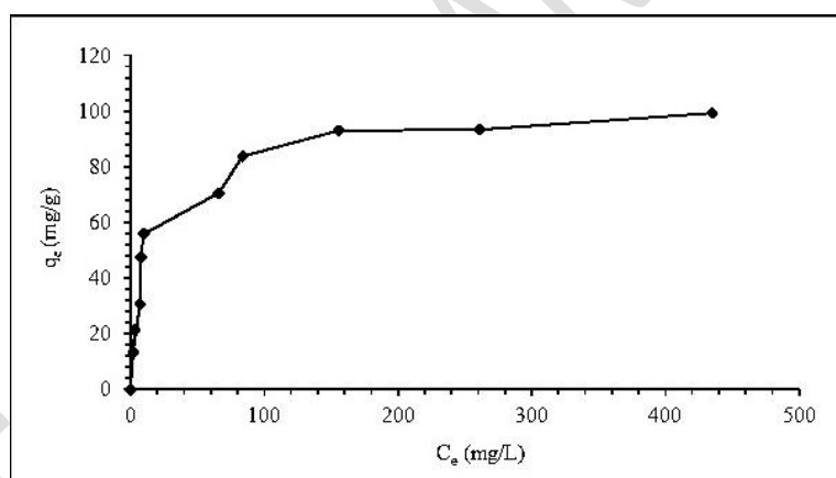
Figure 10: Isotherm of methylene blue adsorption.
