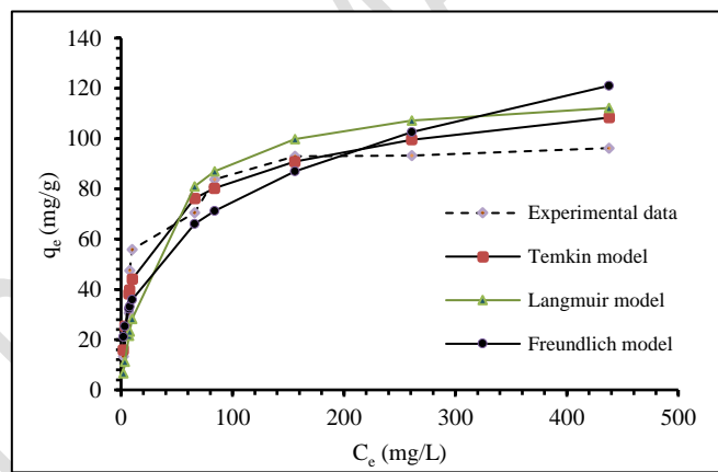
The predicted curve fits for equilibrium isotherms of methylene blue adsorption
