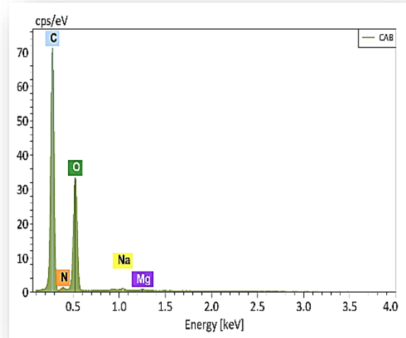
The spectrum EDS
