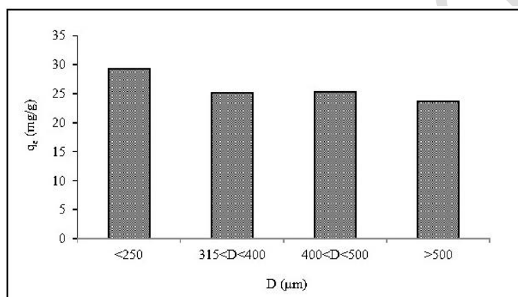
Figure 4: Effect of particle size on methylene blue adsorption onto NaOH-activated peanut shells.
