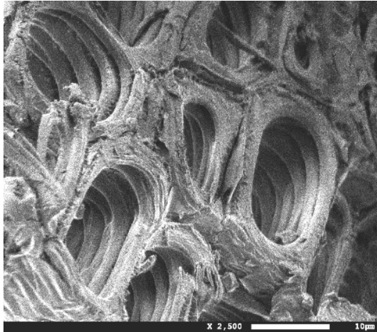
SEM image of NaOH-activated peanut shells
