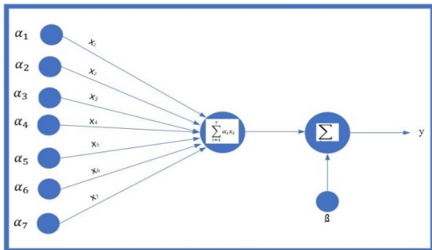
Figure 7. Linear prediction model general representation.
