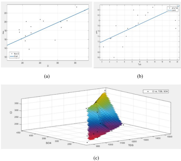
Figure 6. a) Na vs Cl linear regression graph b) pH vs Turb linear regression graph c) Cl vs SO4, TDS linear regression graph.
