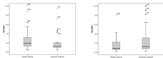
Figure 3. Seasonal variation THg (ng/L) in two areas (a: Thermaikos, b: South Peloponnese)
