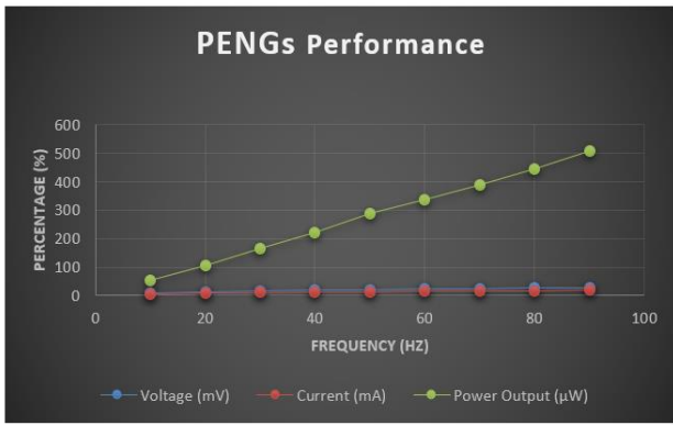
Figure 1. Frequency-Dependent Power Output of PENGs
