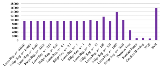
Figure 7. MSE comparison of each estimator for the amount of oil dispersion.
