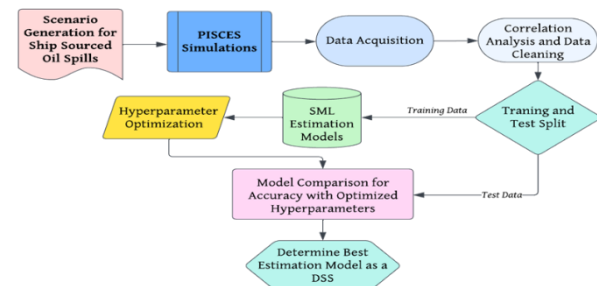
Figure 1. The general framework of the applied methodology.
