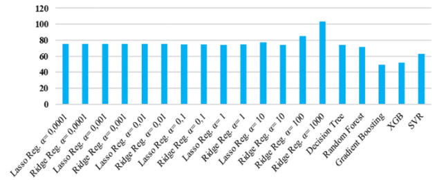
Figure 11. MAE comparison of each estimator for the time of oil impact on shore.
