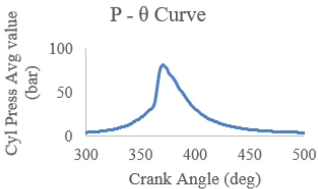
Figure 7.3.2. peak cycle pressure diesel with hydrogen 3ms
