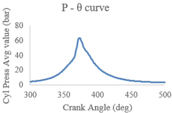
Figure 7.3.1. peak cycle pressure for Diesel
