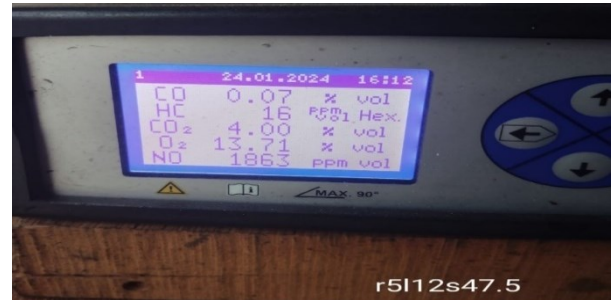
Figure 7.2.5. Emissions diesel with hydrogen at 6ms
