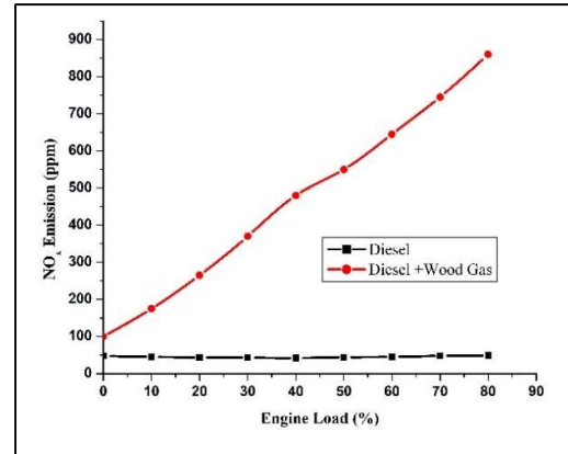
Figure 16: NO x Emission for dual fuels and Diesel
