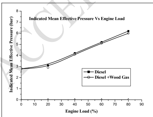
Figure 18: Indicated Mean Effective Pressure with Engine Load
