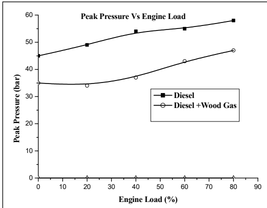
Figure 17: Variations of Peak Pressure with Engine Load
