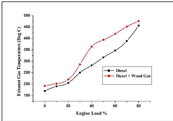
Figure 13: Exhaust Gas Temperatures Vs Engine Load
