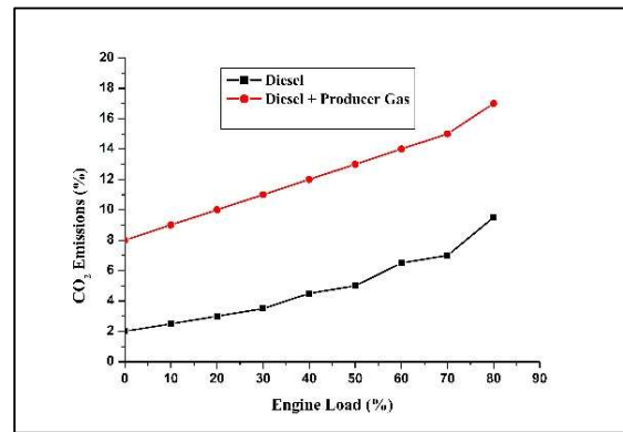
Figure 14: CO2 Emission for dual fuels and Diesel
