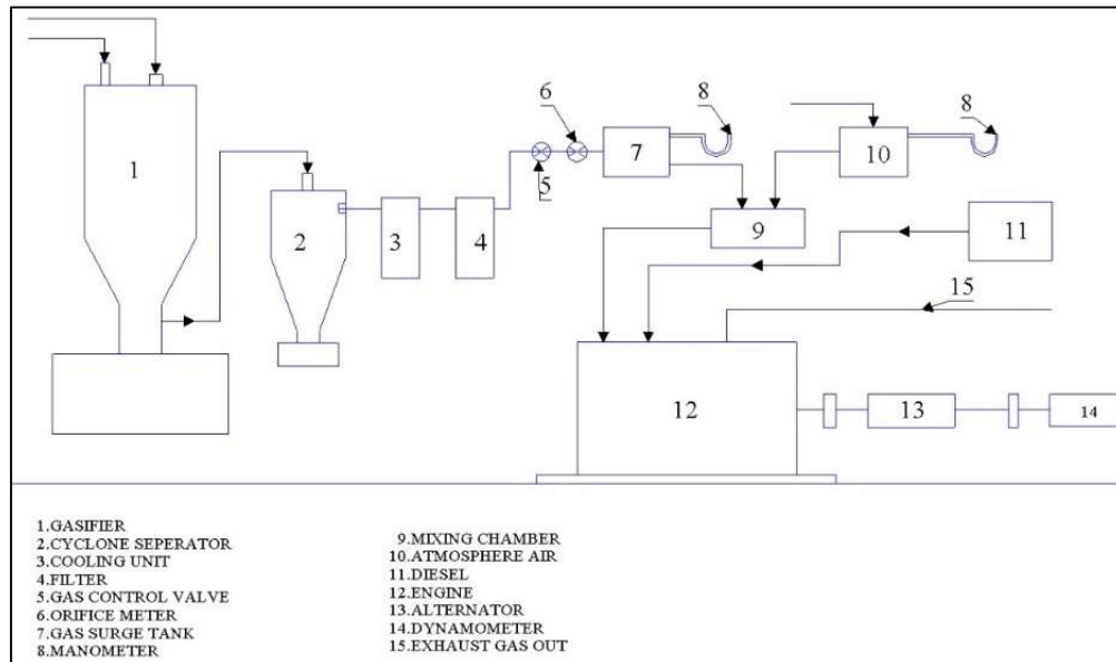
Figure 4: Experimental and Instrumental setup
