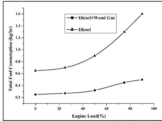
Figure 10: Engine Load Vs Total fuel consumption
