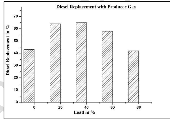
Figure 12: Diesel Replacement with producer gas
