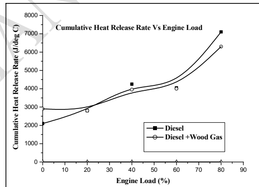
Figure 19: Cumulative Heat Release Rate with Engine Load
