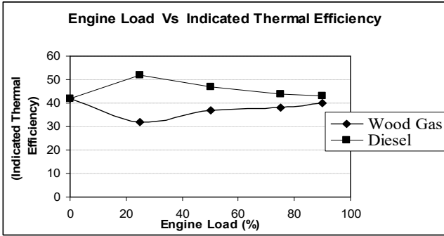
Figure 9: Engine Load Vs Indicated Thermal Efficiency
