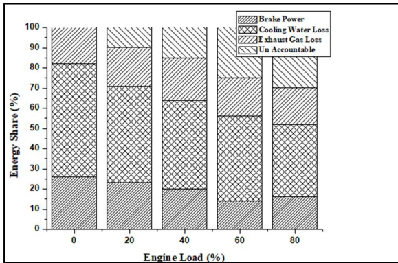
Figure 11: Heat Balance analysis on Diesel and Wood
