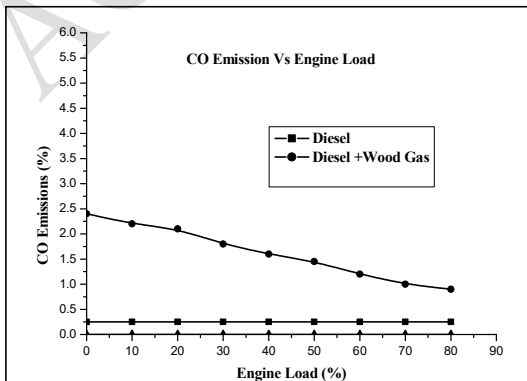
Figure 15: CO Emission for dual fuels and Diesel
