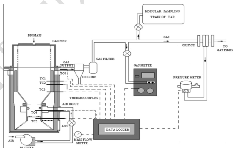
Figure 6b : Gasifier System with measuring instruments.
