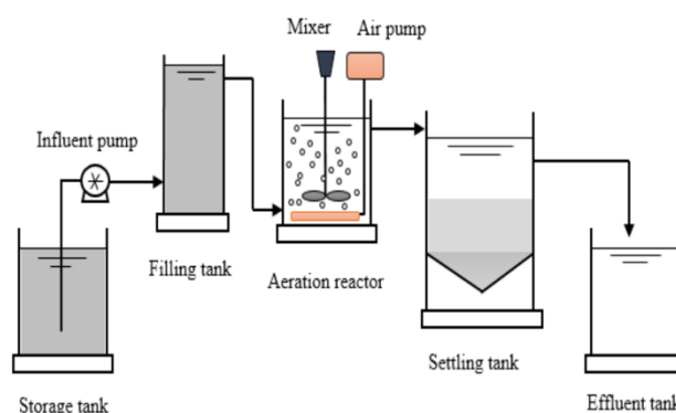
Figure 1. Sequencing Batch Reactor- Schematic Diagram
