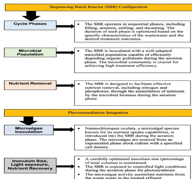
Figure 2. Experimental configuration for combining SBR and phycoremediation
