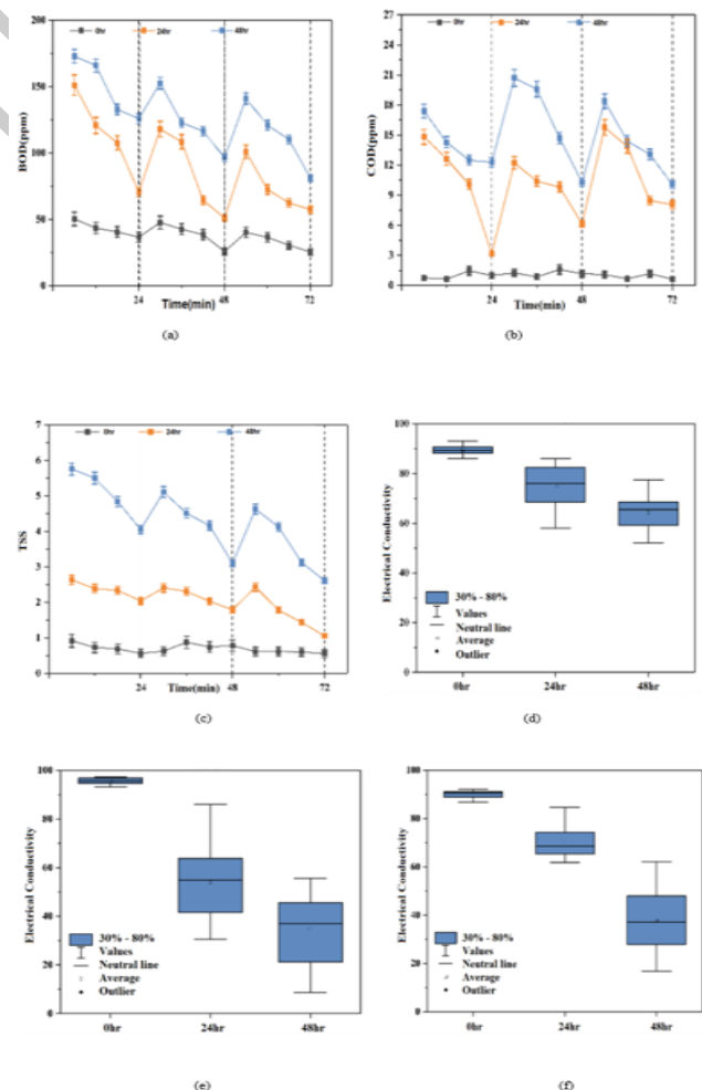
Figure 6. Evaluation of the sequential batch reactor performance
