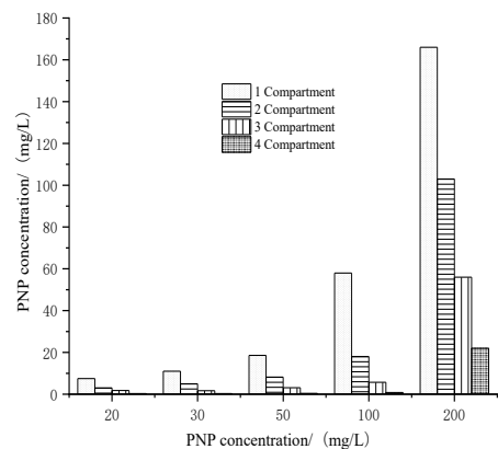
Figure 6. Change of PNP in each compartment of reactor under different PNP concentration
