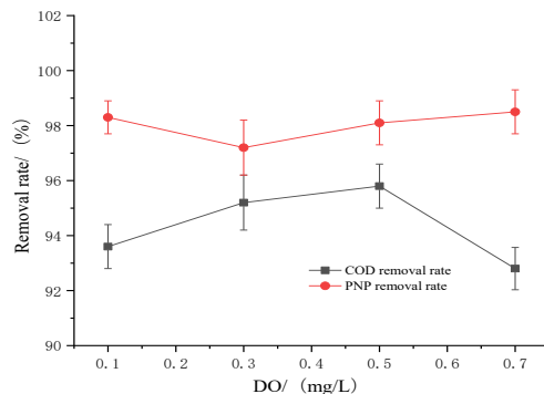
Figure 16. The impact of DO changes on COD and PNP
