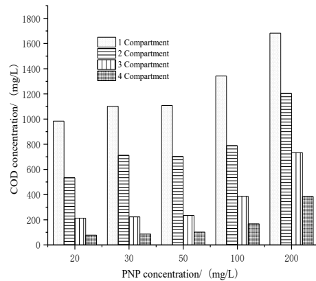
Figure 5. Changes of COD concentration in different compartments under different PNP concentrations
