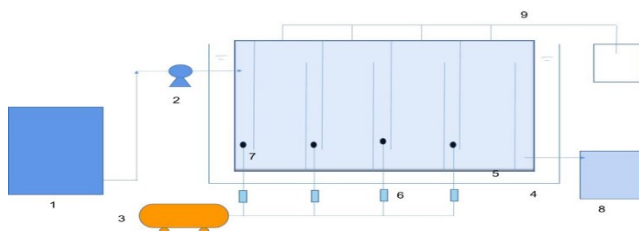
Figure 1. Experimental equipment. 1. Raw water tank, 2. Peristaltic pump, 3. Air pump, 4. Thermostatic water tank, 5. Micro oxygen baffle reactor, 6. Flowmeter, 7. Aerator, 8. Water tank, 9. Gas outlet
