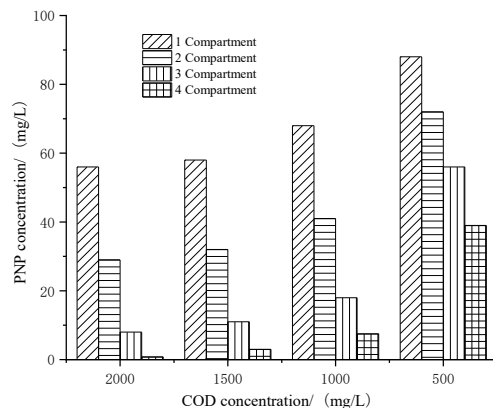
Figure 11. Changes of PNP in each compartment of the reactor under different COD concentrations
