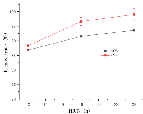
Figure 12. The impact of HRT changes on COD and PNP
