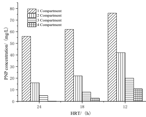
Figure 15. Changes of PNP in each compartment of the reactor under different HRT conditions
