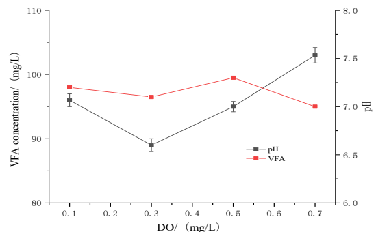
Figure 17. The impact of DO changes on VFA and pH
