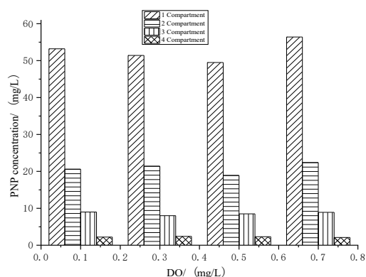
Figure 19. Changes of PNP in each compartment of the reactor under different DO concentration
