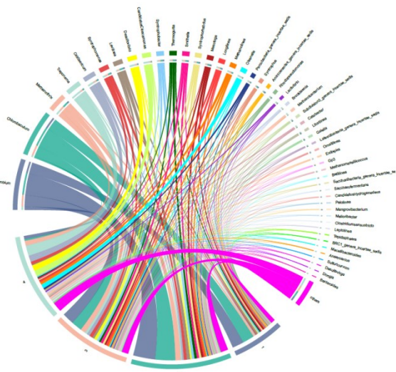
Figure 22. Taxonomic composition distribution in samples at the genus level
