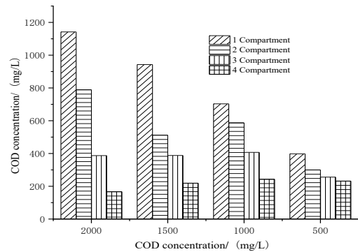
Figure 10. Changes of COD in each compartment of the reactor at different COD concentrations
