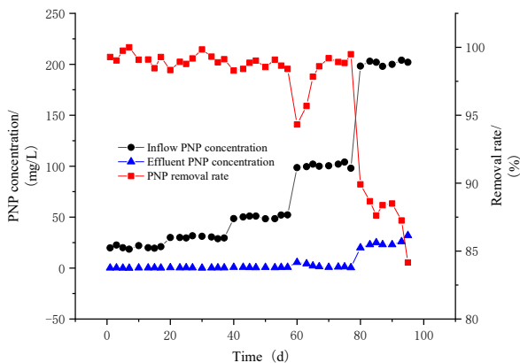
Figure 3. Effect of Influent PNP Concentration on PNP Removal The variation of PNP concentration in the effluent of each compartment is similar to that of COD. When the inlet PNP concentration is 100mg/L, the first compartment of mOBR has a significant increase in PNP concentration in the effluent. Still, the second compartment can degrade PNP to the previous level, indicating that the reactor can
