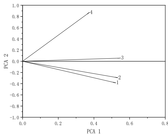
Figure 23. PCA analysis of microbial community structure in each compartment
