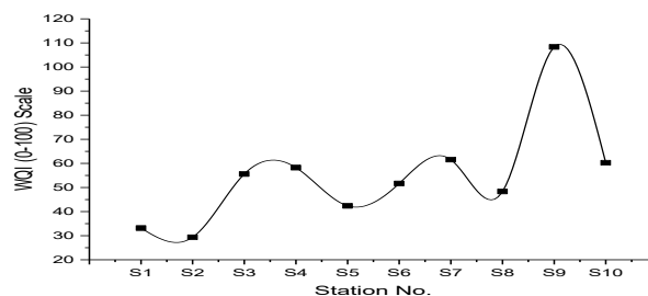
Figure 5. WQI of Noyyal river water at different locations
