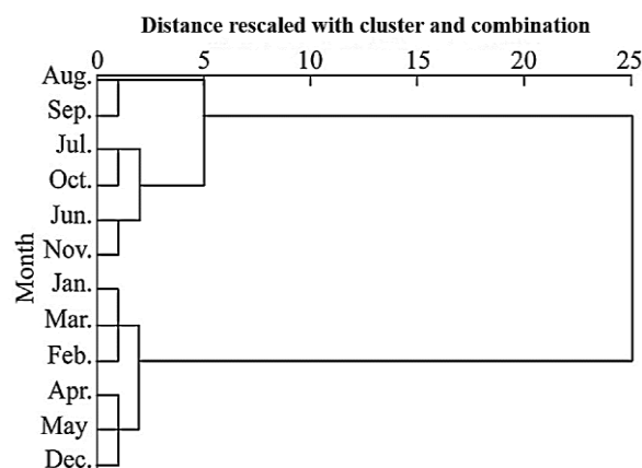
Figure 3. Dendrogram plot of water samples in different months and their hierarchical clustering
