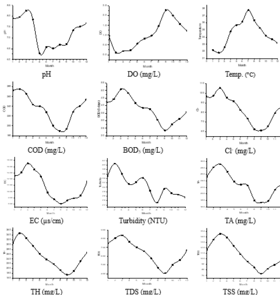
Figure 2. Variations in physical and chemical properties of Noyyal river from Dec 2022 to Nov 2023
