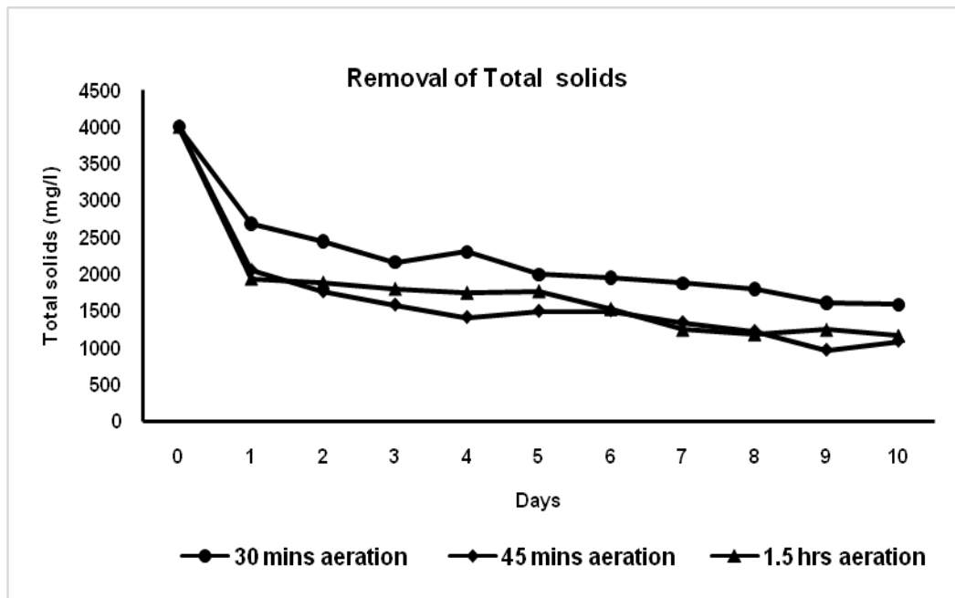
Fig 4 b. Removal of total solids using fujino spiral as biocarrier
