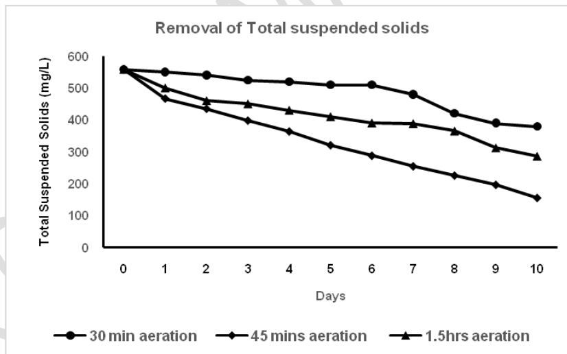
Fig 6 b. Removal of total suspended solids using loofah sponge as bio-carrier
