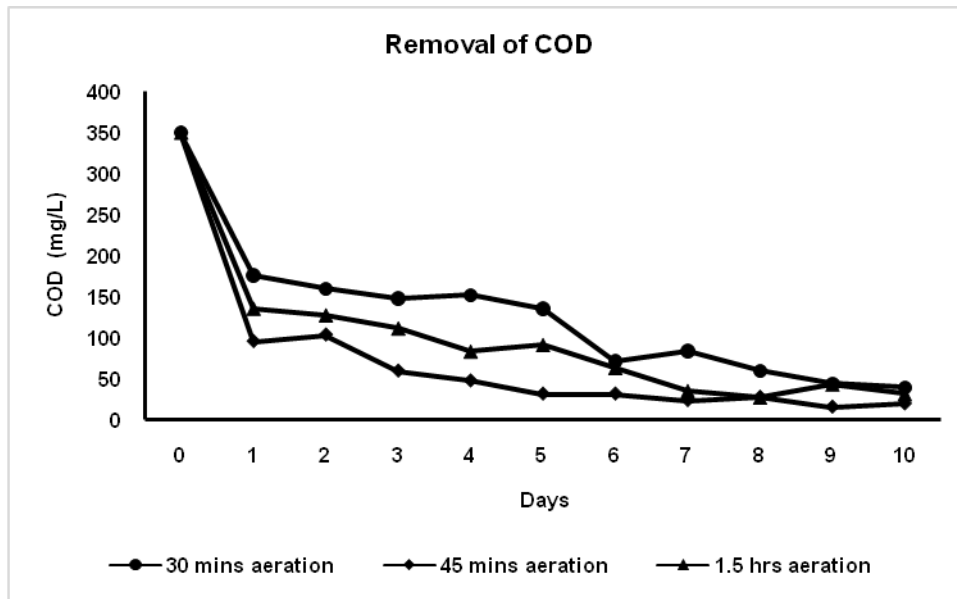
Fig 4 c. Removal of COD using fujino spiral as biocarrier
