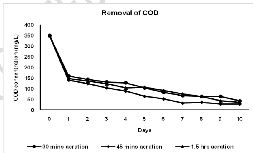
Fig 6 c. Removal of COD using loofah sponge as bio-carrier
