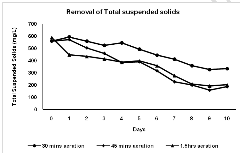
Fig 4 a. Removal of total suspended solids using fujino spiral as biocarrier
