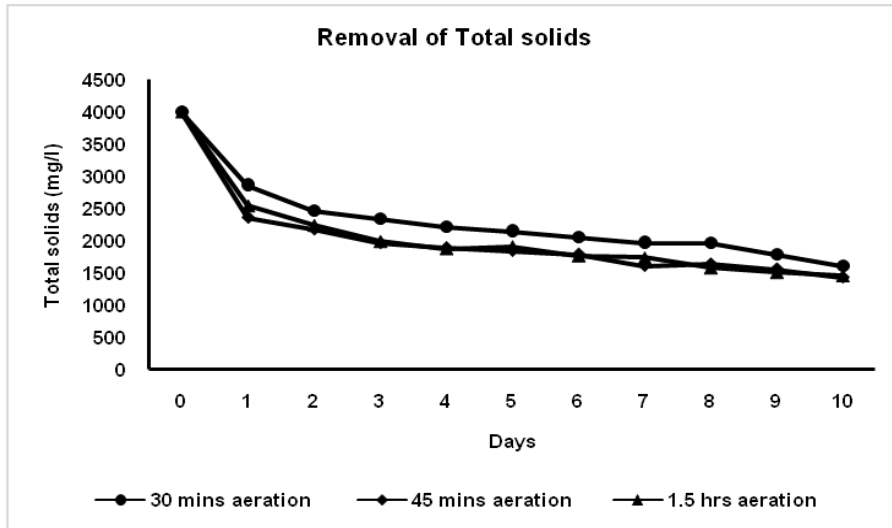
Fig 6 a. Removal of total solids using loofah sponge as bio-carrier
