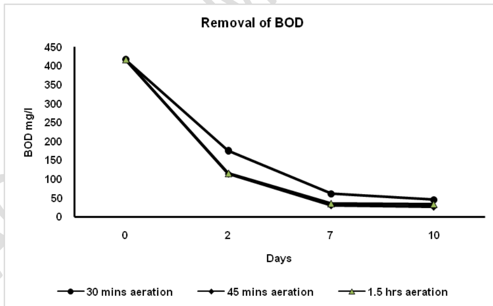
Fig 4 d. Removal of BOD using fujino spiral as biocarrier
