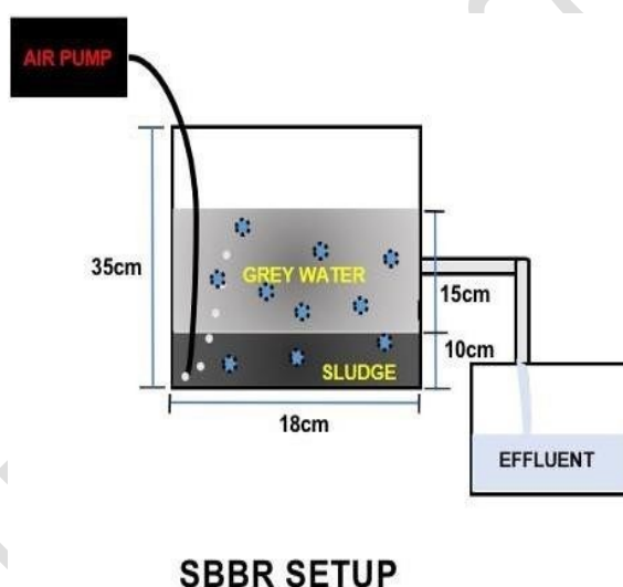
Fig 3. Experimental arrangement of SBBR
