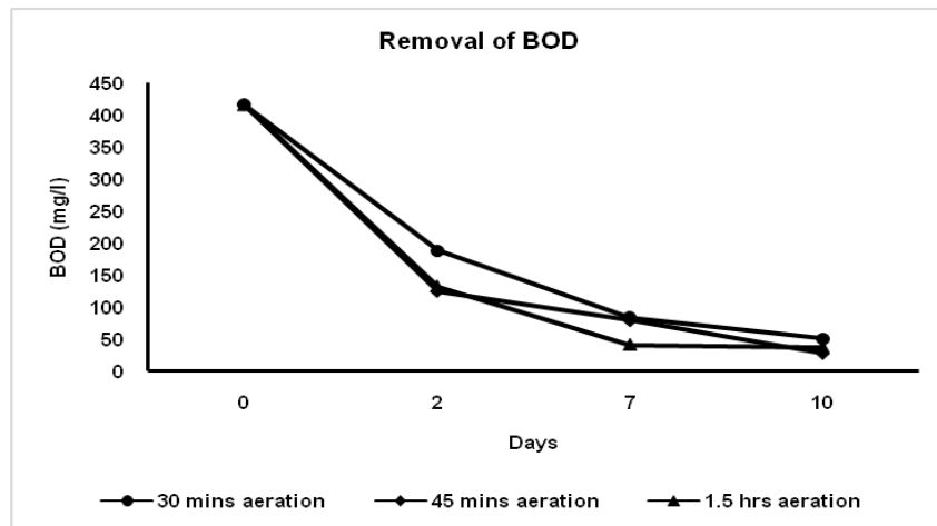
Fig 6 d. Removal of BOD using loofah sponge as bio-carrier
