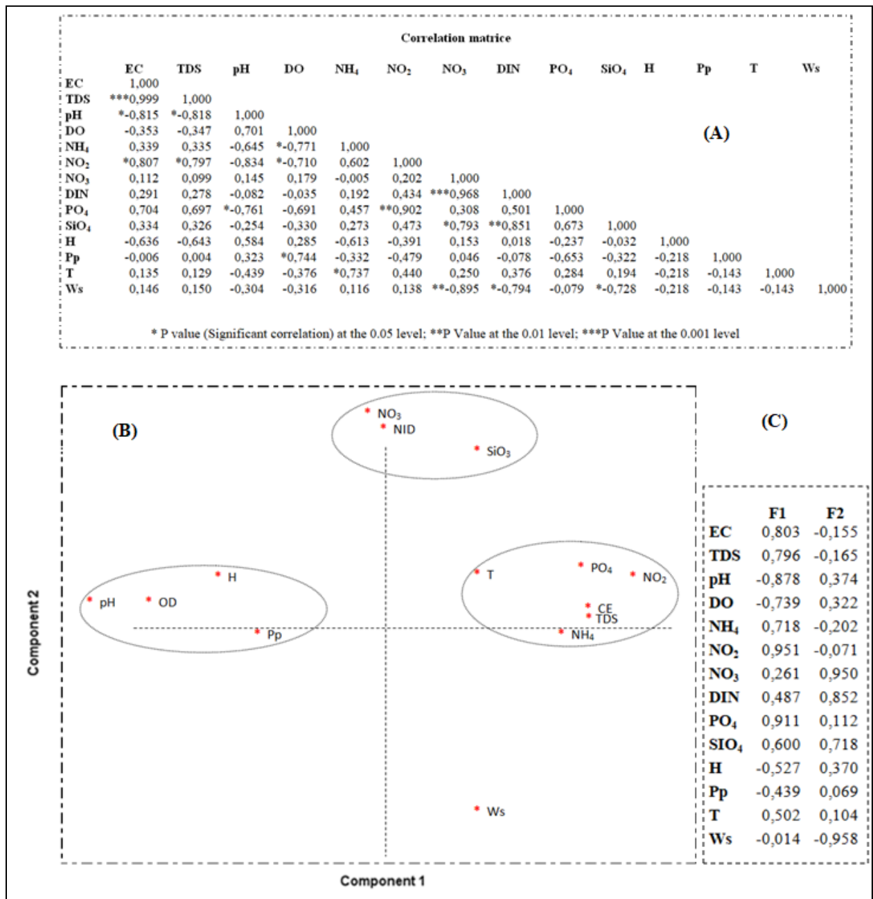
Figure 3. Statistical analysis results. (A): Correlation matrix of the physicochemical parameters of water samples; (B): Factorial plan projection 1 \times 2 of principal component analysis; (C): Factorial charges and variance explained in the factorial analysis of the variables assessed, after rotation using the varimax method.
