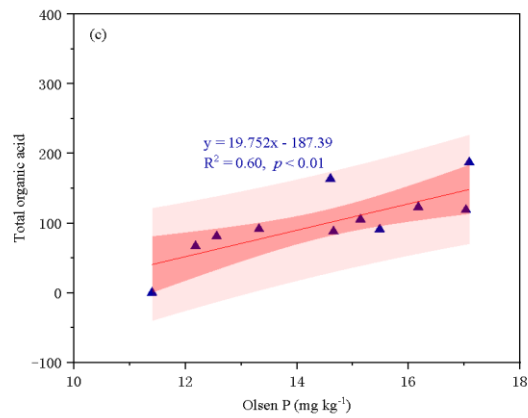
Figure 5. Relationships between soil available P (Olsen P) and Fe-P and O-P contents (a), pH (b) and total organic acid content (C)
