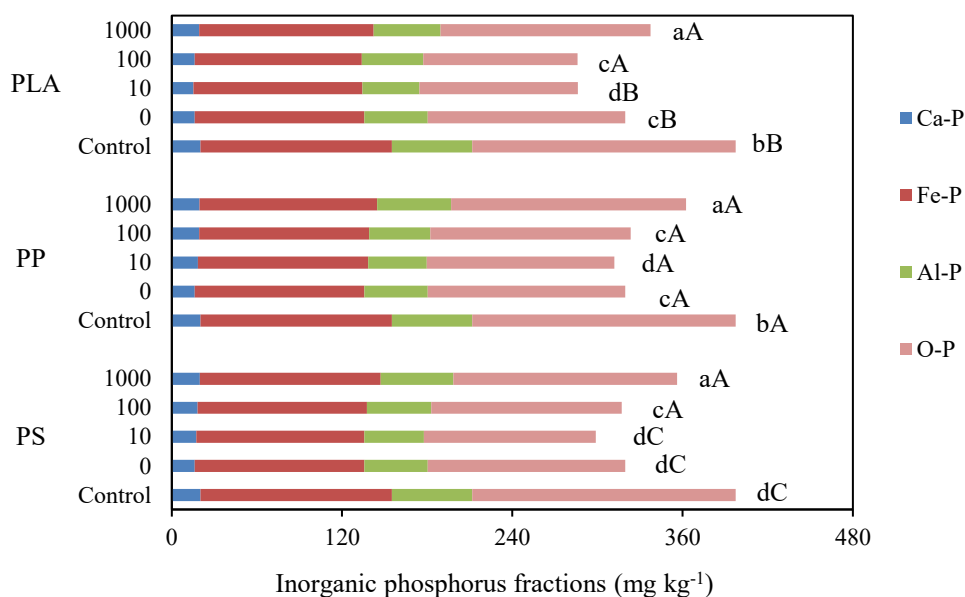
Figure 3. Variations of soil inorganic P fractions
