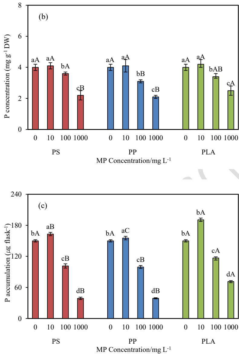
Figure 1. Effects of three MPs on the biomass (a), P content (b) and uptake capacity (c) of the Ld mycelium.
