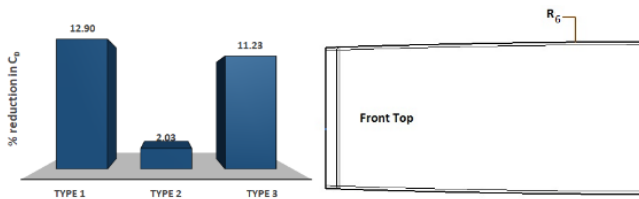
Figure 15. Side Panels curvatures, R_6 vs % reduction in C_D
