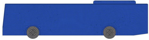
Figure 3. Finite Elements over the bodywork.
