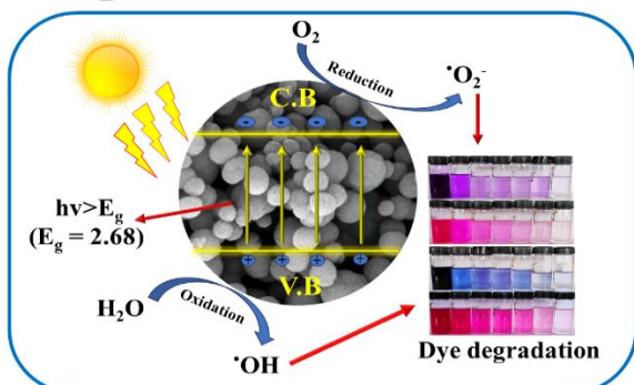
Figure 14. Photocatalytic mechanism of AgO NPs
