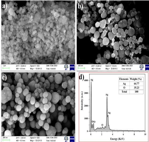
Figure 4. Morphology and primary composition of AgO NPs
