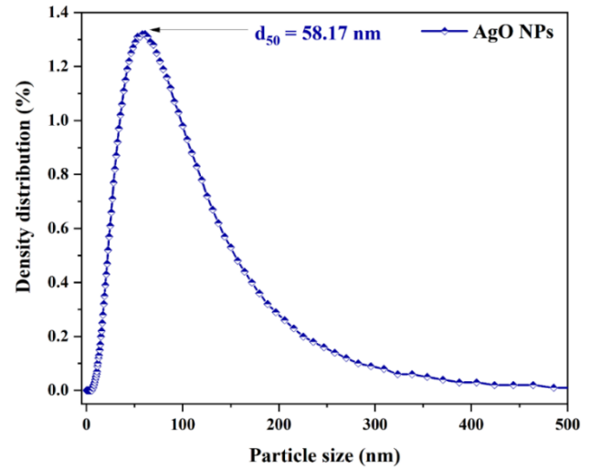
Figure 5. Particle size analysis of AgO NPs
