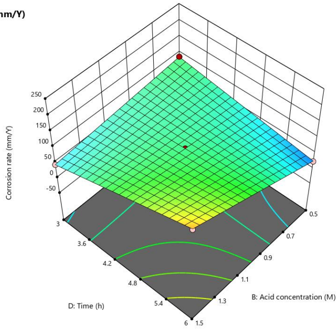
Fig. 6e 3D contour plot depicting the impact of time and acid concentration on corrosion rate
