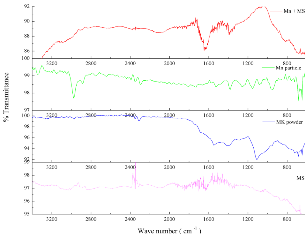
Fig. 2 FTIR spectra of MnOnps
