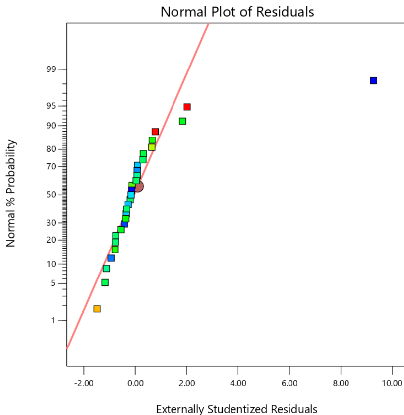
Fig. 5 Normal plot of corrosion rate (expected vs. actual)
