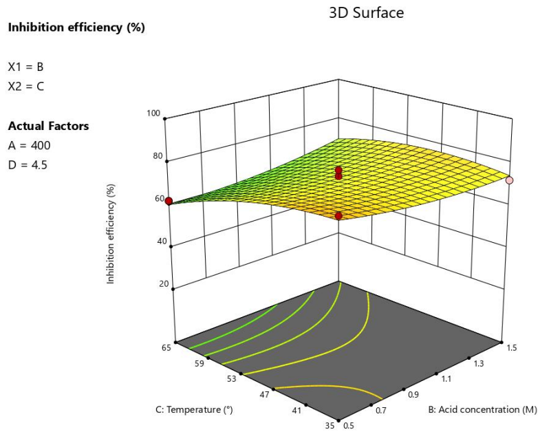
Fig.8d 3D contour plot depicting the impact of temperature and acid concentration on the inhibition efficiency
