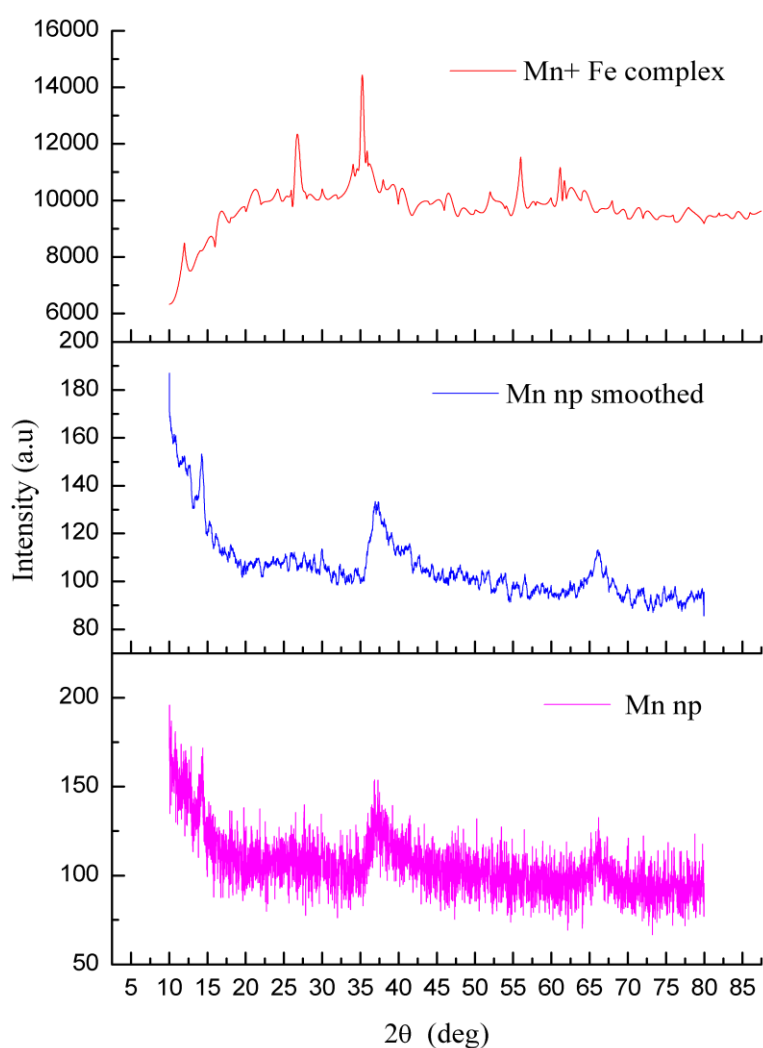
Fig. 3 XRD pattern of MnOnps
