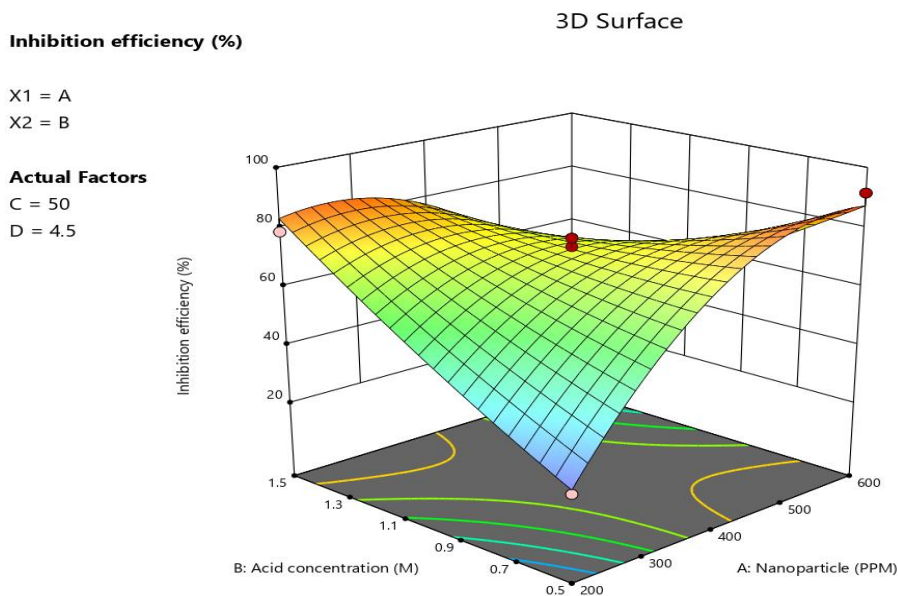
Fig.8a 3D contour plot depicting the impact of acid concentration and nanoparticle dosage on the inhibition efficiency
