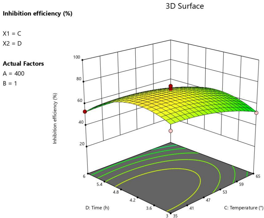
Fig.8f 3D contour plot, depicting the impact of time and temperature on the inhibition efficiency
