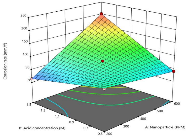
Fig. 6a 3D contour plot depicting the impact of acid concentration and nanoparticle dosage on corrosion rate
