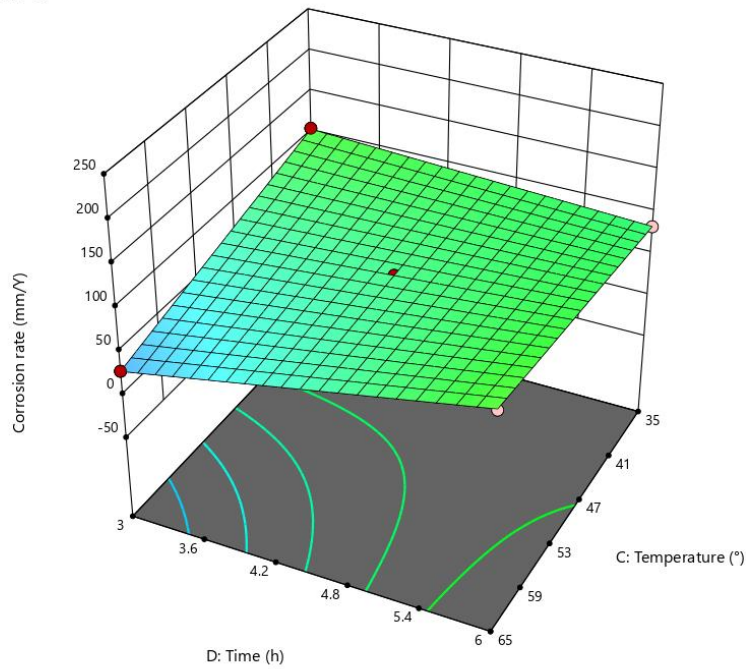
Fig. 6f 3D contour plot depicting the impact of time and temperature on corrosion rate
