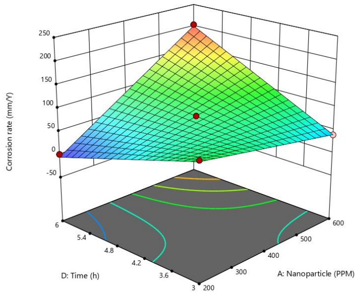
Fig. 6c 3D contour plot depicting the impact time and nanoparticle dosage on corrosion rate
