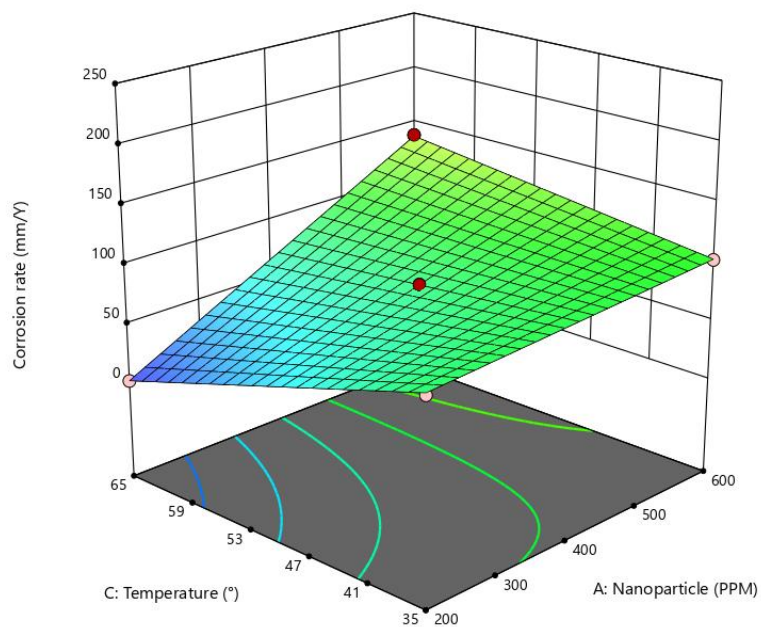
Fig. 6b 3D contour plot depicting the impact of temperature and nanoparticle dosage on corrosion rate
