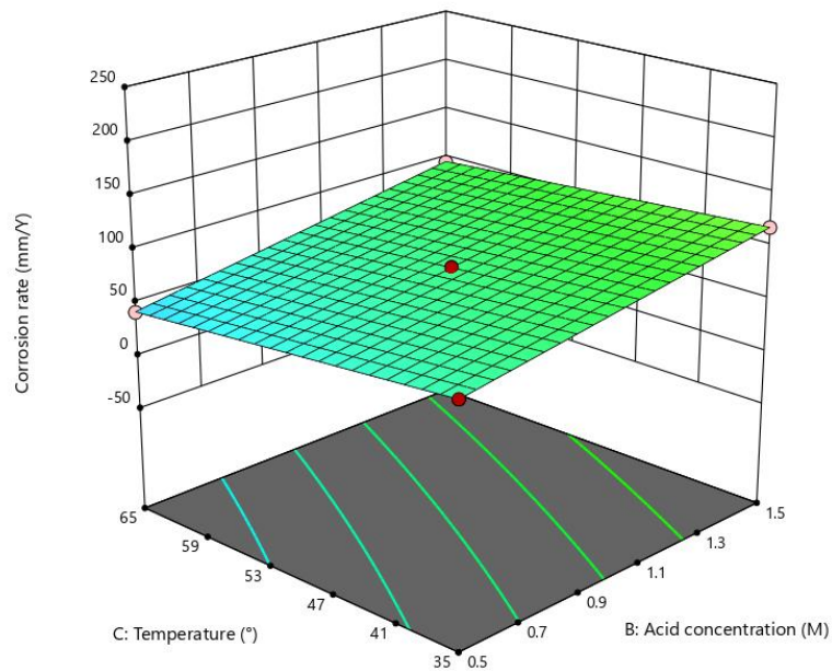
Fig. 6d 3D contour plot depicting the impact of temperature and acid concentration on corrosion rate
