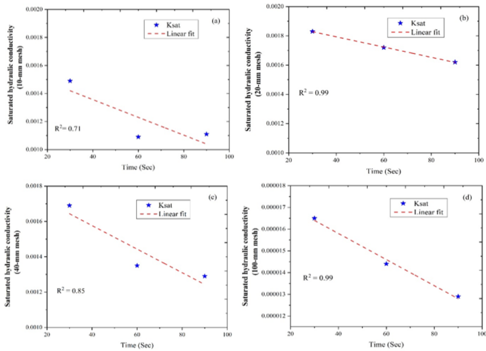
Figure 7. The correlation between Ksat and the falling head method is investigated with different time stages for samples of 10, 20, 40, and 100mm mesh.
