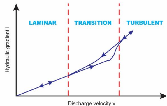
Figure 1. Different zones of turbulent and laminar flow
