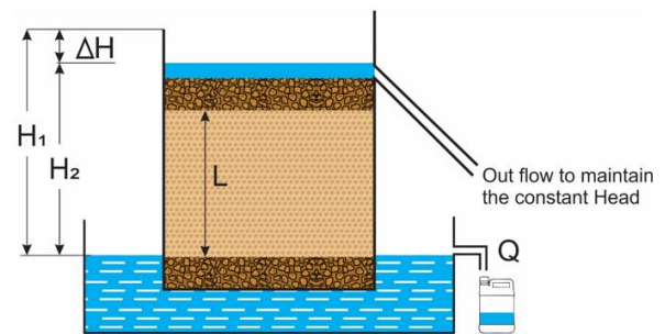
Figure 5. Demonstrates the measurement of the saturated hydraulic conductivity using falling head method
