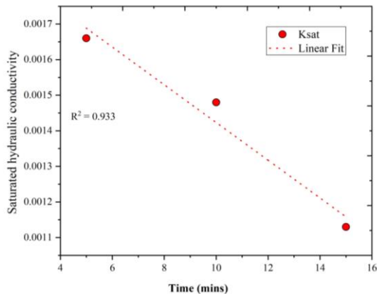
Figure 6. The constant head approach used to measure the hydraulic conductivity with different stages of time samples passed through 10, 20, and 40mm mesh range
