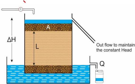
Figure 4. Demonstrates the measurement the saturated hydraulic conductivity using constant head method
