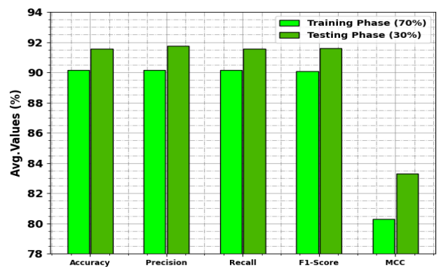
Figure 5. Average of WQIPC-HTDL approach under 70:30 of TRAPH/TESPH
