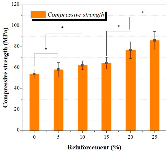
Figure 9. Compressive strength of SS-filled PLA composites
