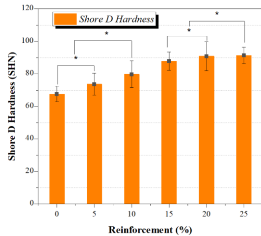
Figure 11. Shore D hardness of SS-filled PLA composites
