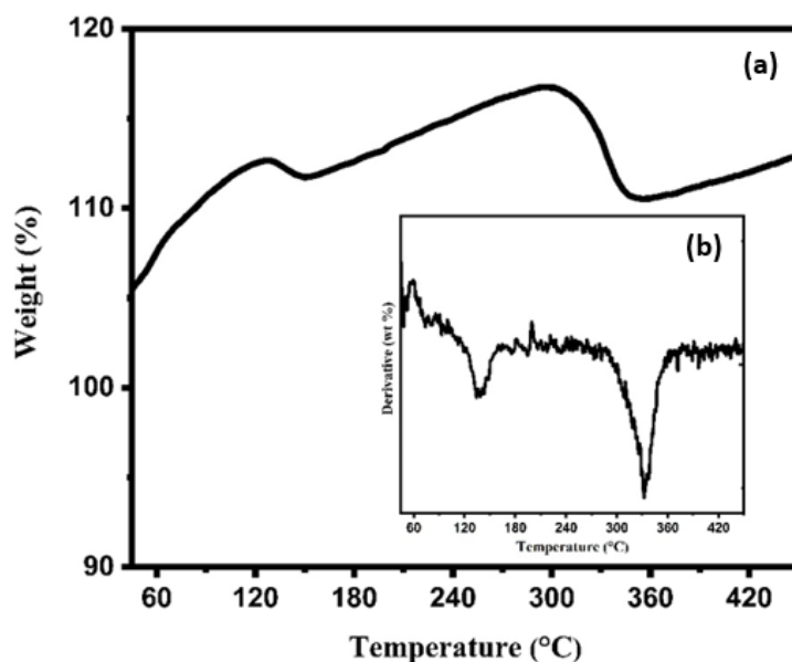
Figure 3. TGA- DTA pattern of CS- ZnO NPs
