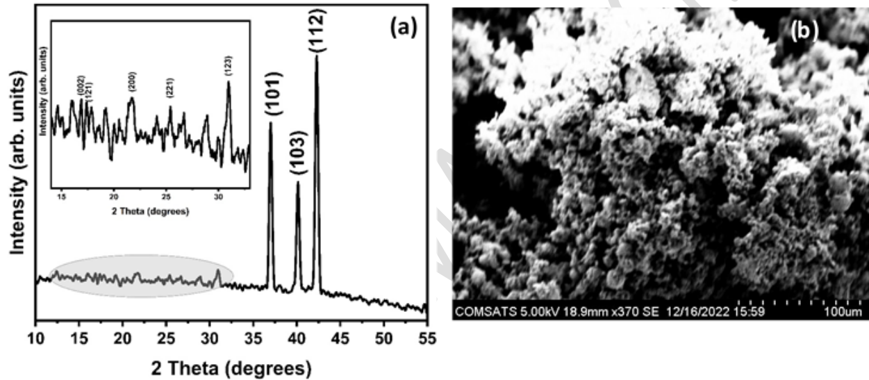
Figure 1. XRD pattern (a) and SEM image (b) of CS-ZnO NPs
