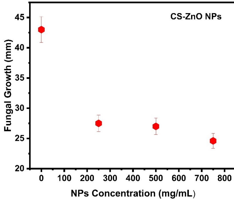
Figure 5. Antifungal activity CS-ZnO NPs against Alternaria solani .
