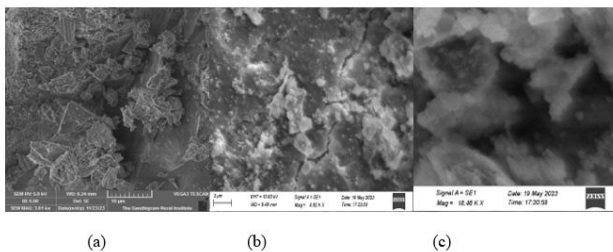
Figure 3. SEM image (a) LA (b) RA (c) CRA
