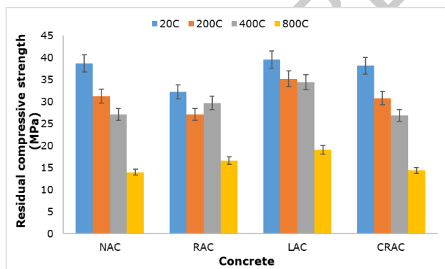
Figure 10. Variation in CS upon elevated temperature
