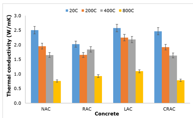
Figure 13. Thermal conductivity
