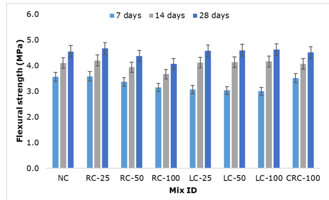
Figure 8. Flexural strength
