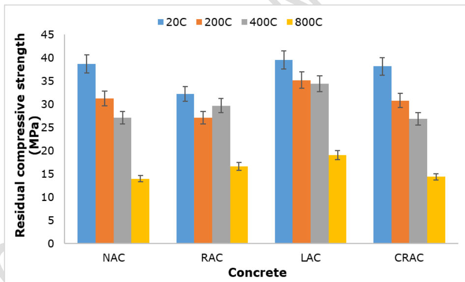
Figure 10. Variation in CS upon elevated temperature
