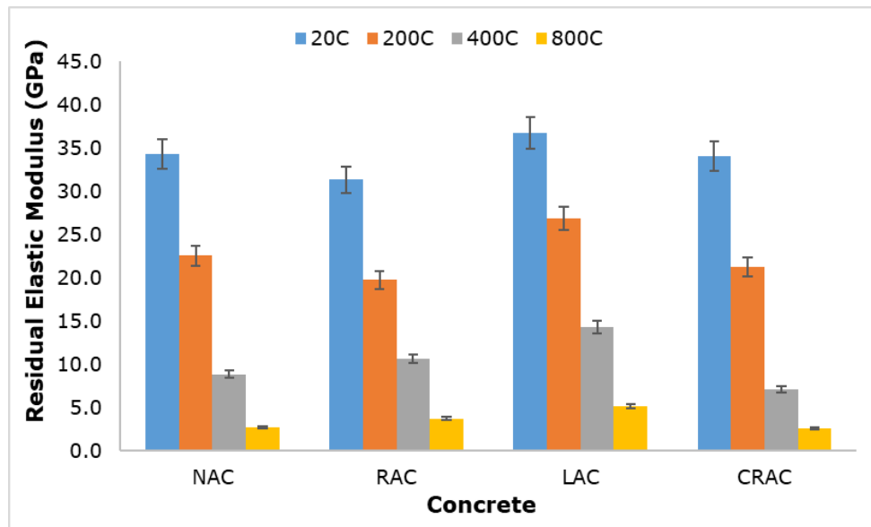
Figure 12. Variation in EM upon elevated temperature
