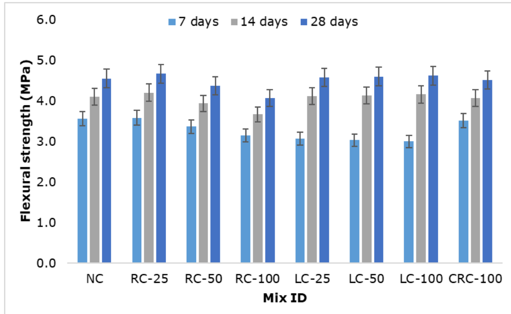
Figure 8. Flexural strength
