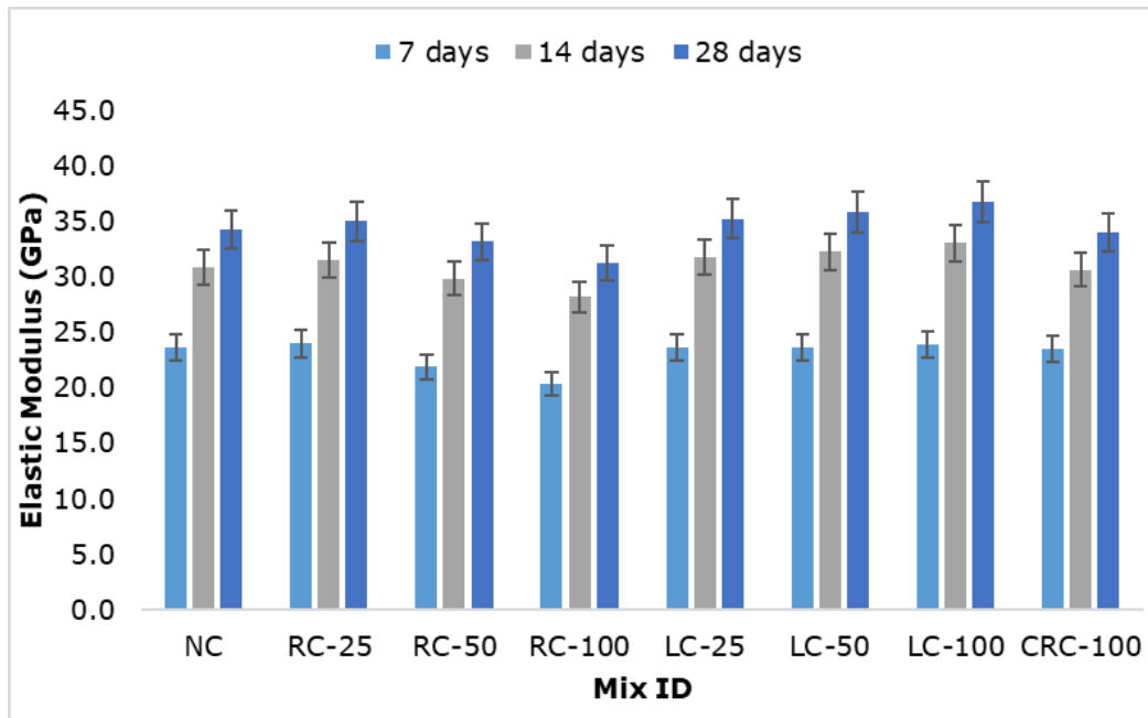
Figure 9. Elastic Modulus
