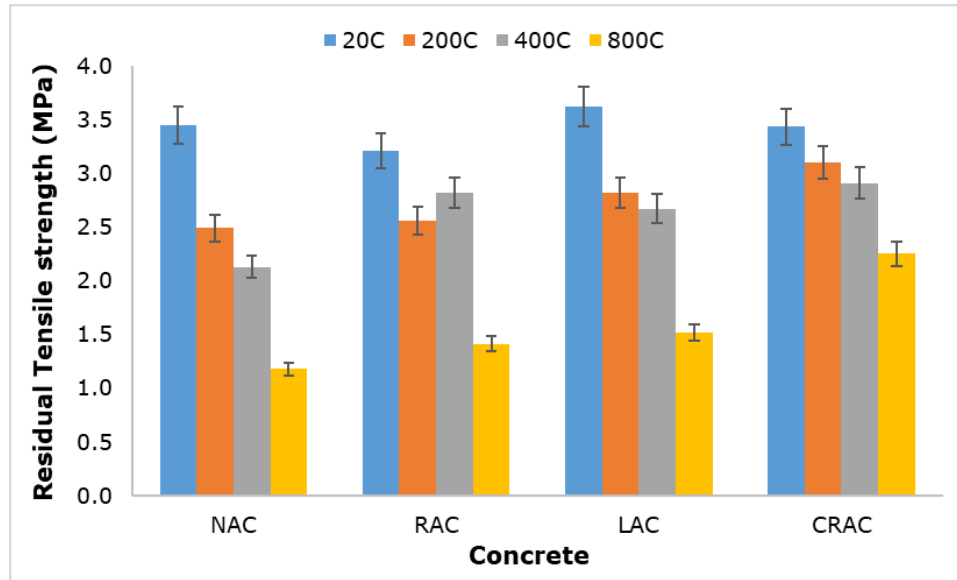
Figure 11. Variation in TS upon elevated temperature
