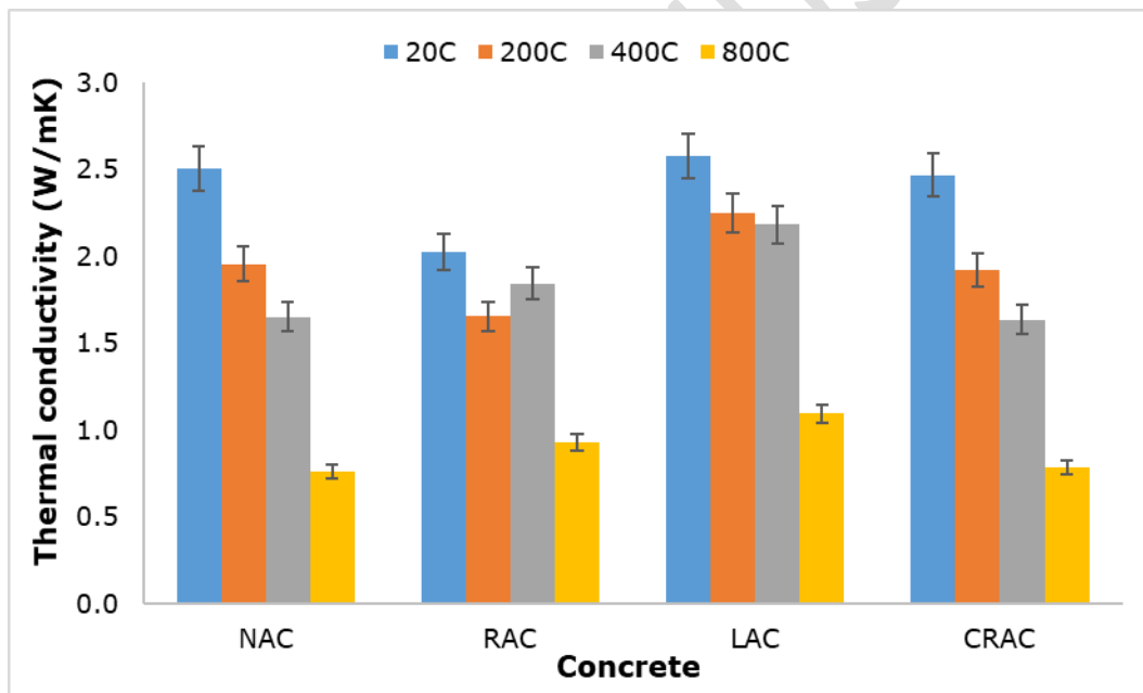
Figure 13. Thermal conductivity
