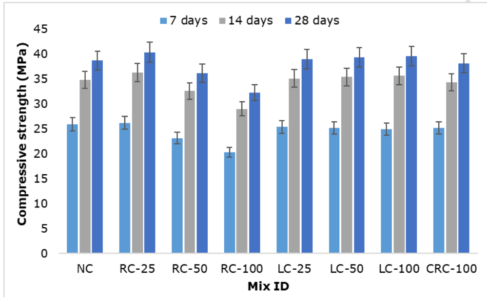
Figure 6. Compressive strength
