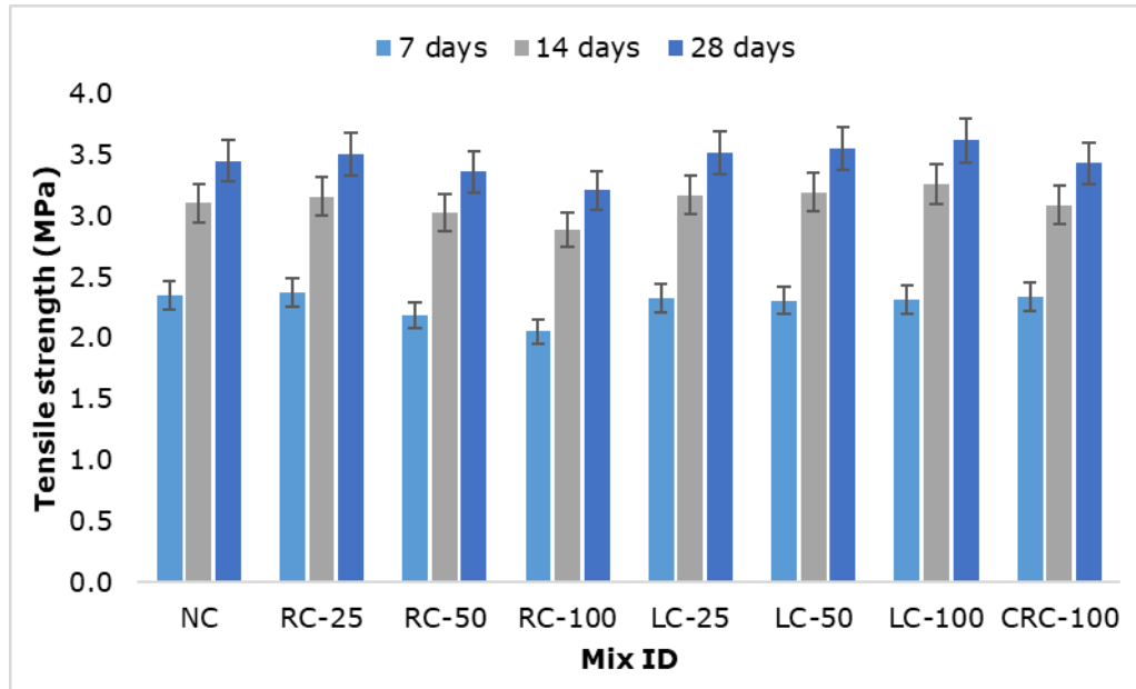
Figure 7. Tensile strength
