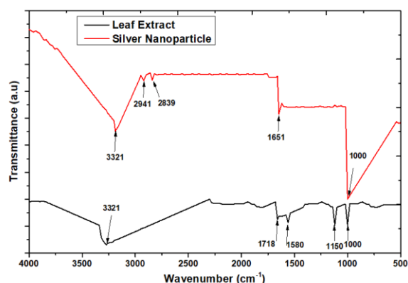
Figure 4. FTIR analysis of biosynthesized Silver Nanoparticles from Lawsonia inermis leaf extract
