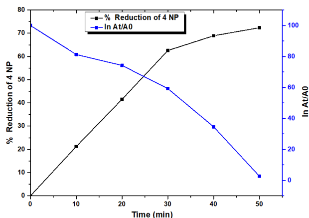
Figure 6. Rate of decrease and \ln(A_t/A_0) plot of 4NP at a catalyst concentration of 0.45 mg/mL of LI-AgNPs
