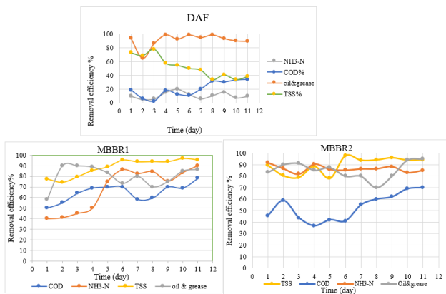
Figure 3. Adaptation phase of DAF-MBBRs
