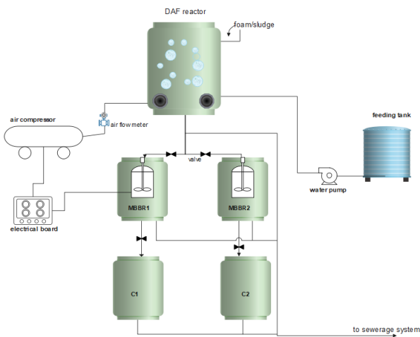
Figure 2. Experimental pilot plant of DAF-MBBR
