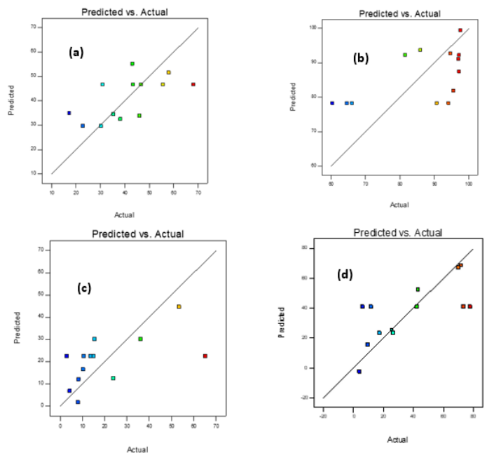
Figure 13. Predicted versus actual plots for DAF (a) COD% (b) oil & grease% (c) Ammonia% and (d) TSS%
