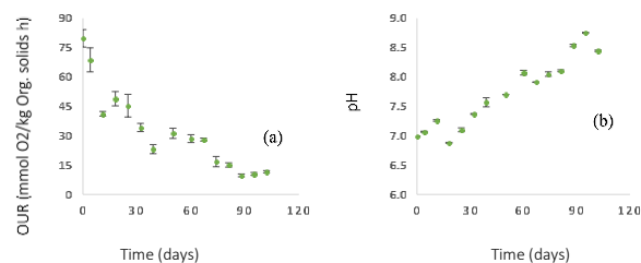
Figure 3. Oxygen uptake rate (a), pH (b) during the main composting process
