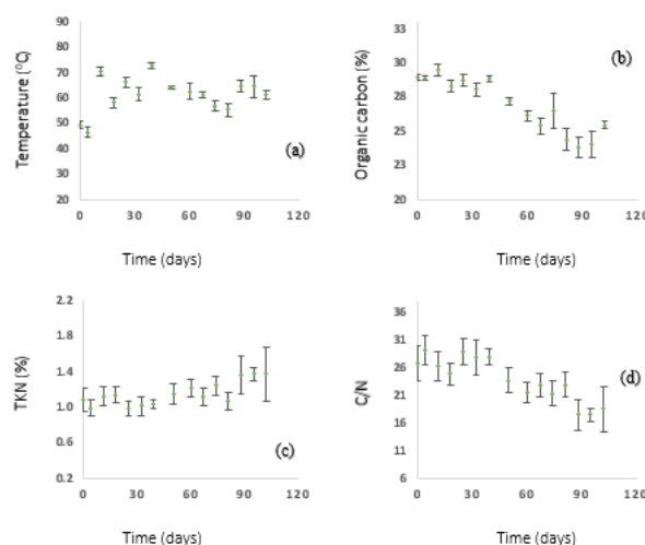
Figure 2. Temperature (a), organic carbon (b), total Kjeldahl nitrogen (c) and carbon to nitrogen ratio (d) during the main composting process
