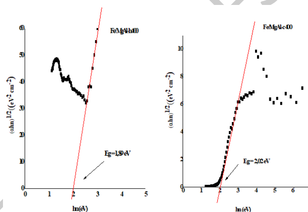
Figure 5. Band gap energies of calcined Fe/MgAl-h400 and Fe/MgAl-c400
