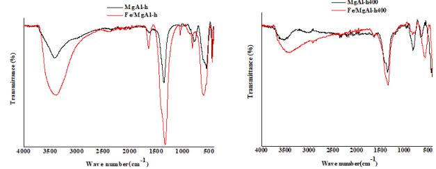
Figure 2. FTIR spectra of the not calcined MgAl-h and calcined Fe/MgAl-h400
