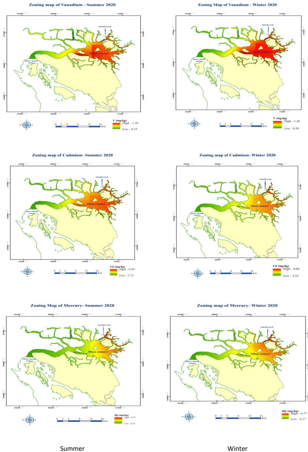
Figure 2. Zoning of heavy metal concentrations in the Musa Estuary
