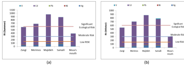
Figure 3. Results of RI index in Mahshahr estuaries in summer and winter 2019. (a). Summer (b). Winter
