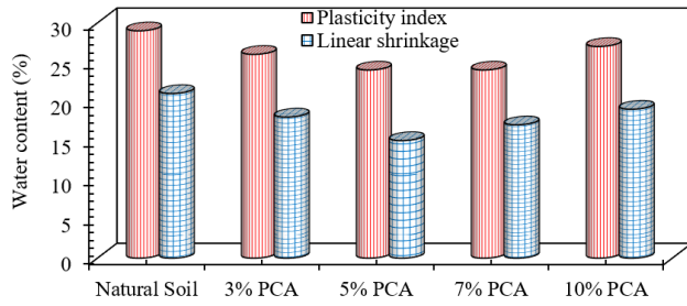
Figure 3. PI and LS values of natural and PC ash-treated soils
