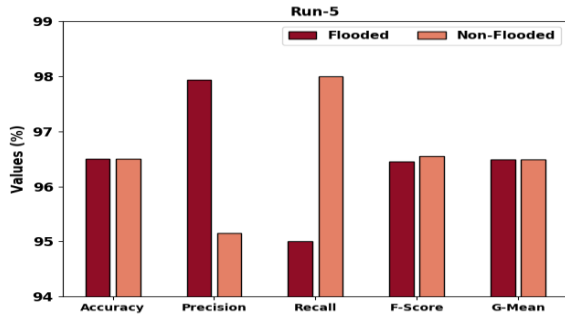
Figure 9. Result analysis of MVODTL-FD approach under run5
