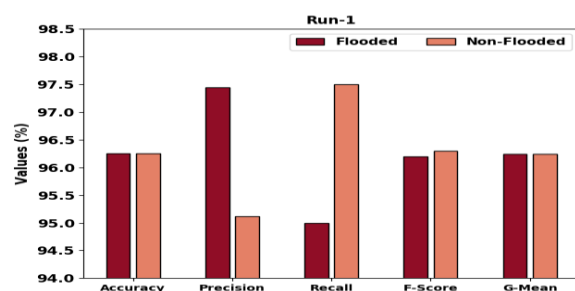
Figure 5. Result analysis of MVODTL-FD approach under run1
