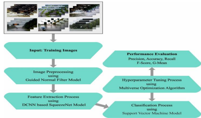
Figure 1. Block diagram of MVODTL-FD approach
