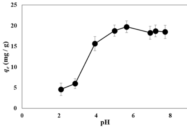
Figure 1. Effect of pH on adsorption of MB on FL. Experimental conditions: contact time 24 h, initial metal concentration 50 mg/L, adsorbent/solution ratio 0.1 g/0.05 L, agitation rate 125 rpm, temperature 295 K
