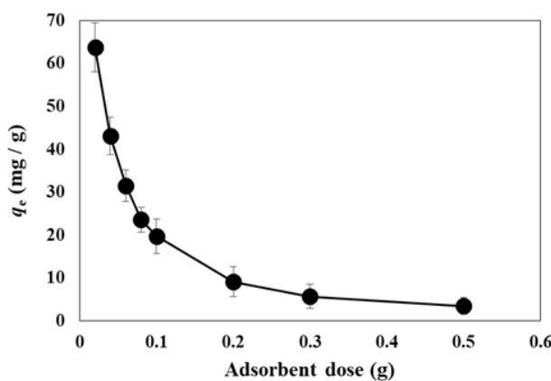
Figure 2. Effect of adsorbent dose on adsorption of MB on FL. Experimental conditions: pH 5.6, contact time 24 h, initial metal concentration 50 mg/L, volume 0.05 L, agitation rate 125 rpm, temperature 295 K
