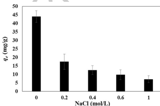
Figure 5. The effect of solution ionic strength (NaCl concentration ranged from 0 to 1 mol/L) on the adsorption of MB by FL. Experimental conditions: pH 5.6, initial concentration 50 mg/L, contact time 24 h, adsorbent/solution ratio 0.04 g/0.05 L, agitation rate 125 rpm, temperature 295 K
