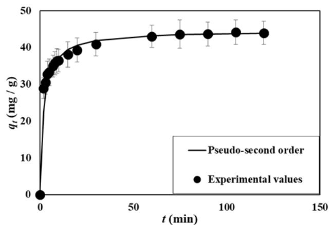
Figure 3. Effect of contact time on adsorption of MB on FL. Experimental conditions: pH 5.6, initial metal concentration 50 mg/L, adsorbent/solution ratio 0.04 g/0.05 L, agitation rate 125 rpm, temperature 295 K
