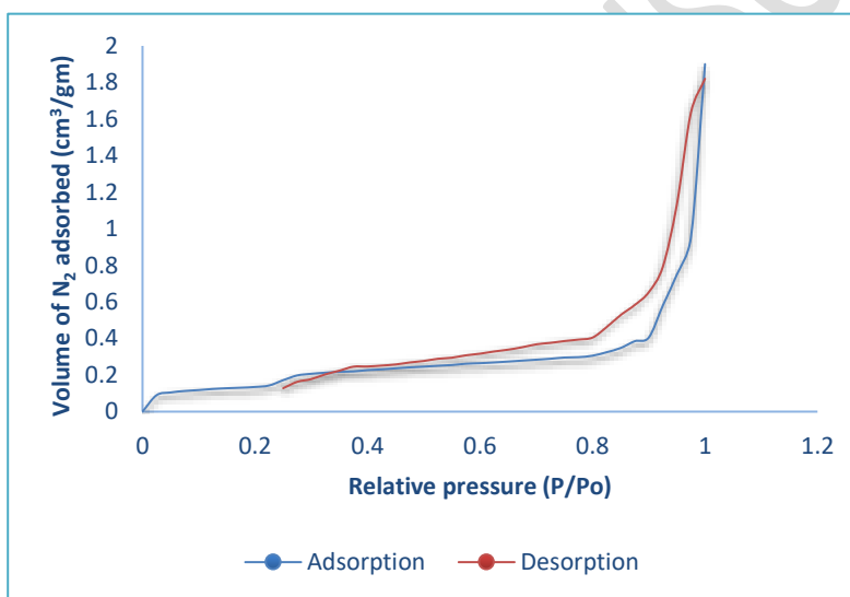
Figure 2 – Surface area analysis of neem leaf biosorbent
