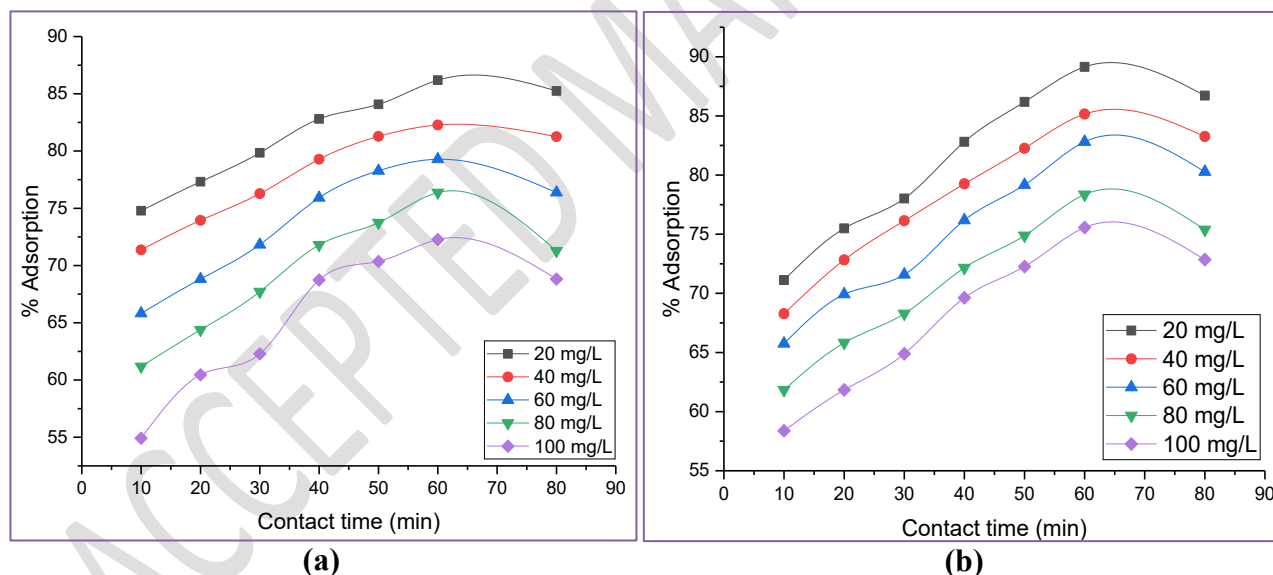
Figure 7 – Changes in adsorption efficiency by altering Contact time for (a) As & (b) Cr metal ions
