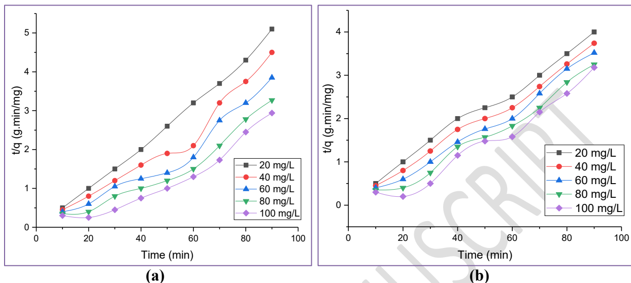
Figure 15 – Pseudo second order plots for the adsorption of (a) As & (b) Cr heavy metal ions using neem leaf biosorbent
