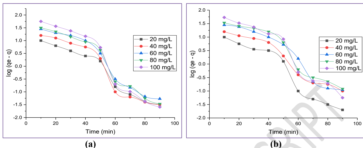
Figure 14 – Pseudo first order plots for the adsorption of (a) As & (b) Cr heavy metal ions using neem leaf biosorbent
