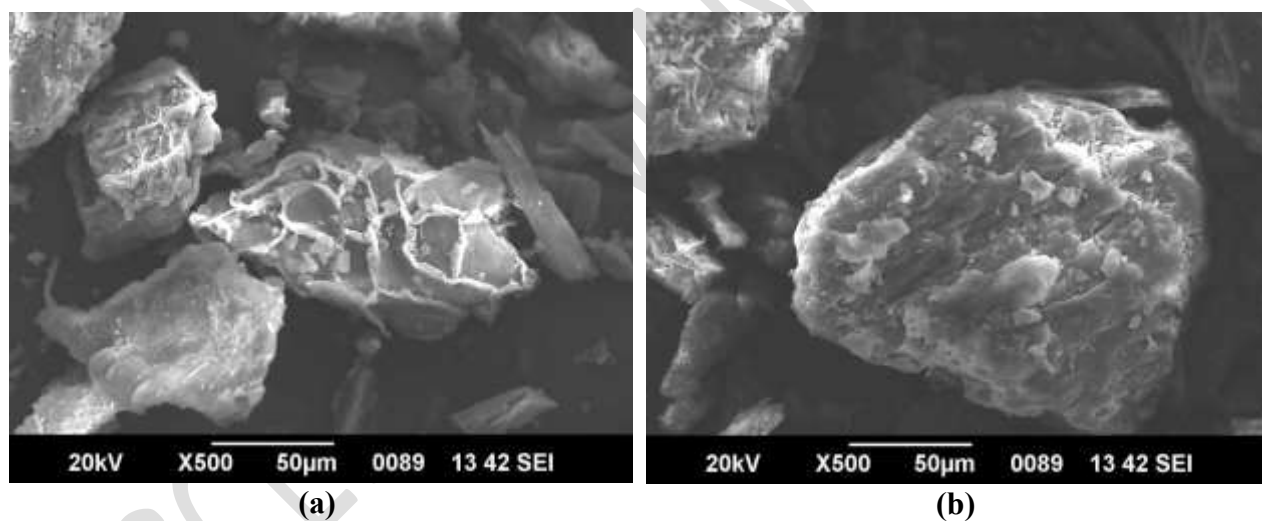
Figure 3 – Scanning Electron Microscope analysis of neem leaf biochar (a) Raw & (b) Metal ions loaded respectively
