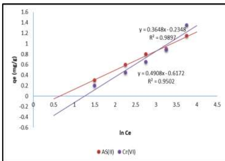
Figure 12 – Temkin isotherm plot for heavy metal adsorption using biochar made from neem leaves
