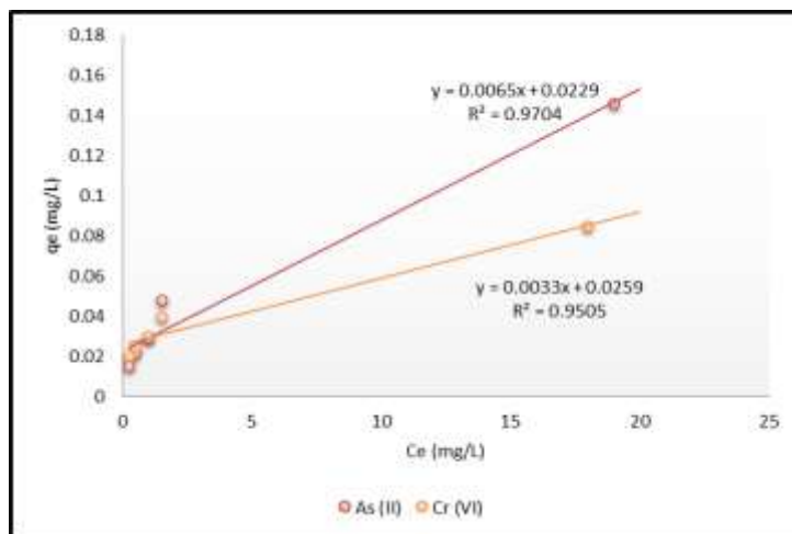
Figure 10 – Langmuir isotherm plot for the adsorption of heavy metals using neem leaf biochar
