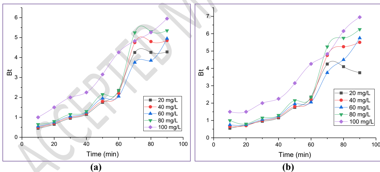
Figure 16 – Boyd kinetic plots for the adsorption of (a) As & (b) Cr heavy metal ions using neem leaf biosorbent
