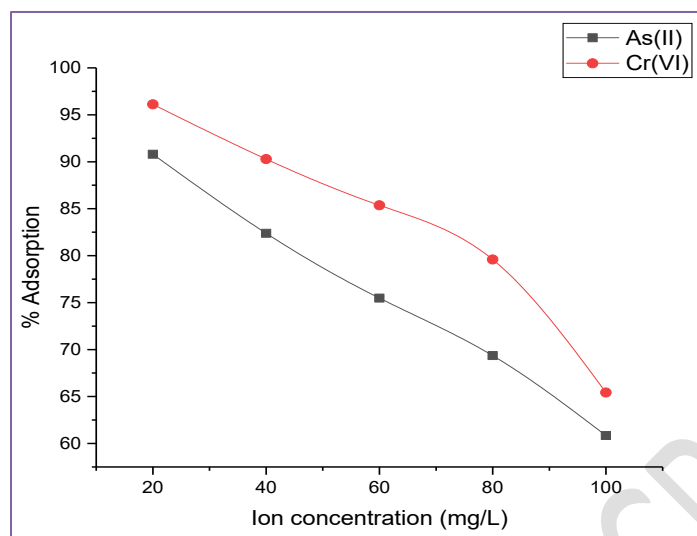
Figure 8 – Adsorption efficiency modifications caused by changing metal ion concentrations
