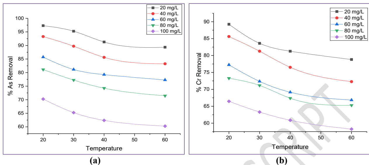
Figure 9 – Changes in adsorption efficiency by varying solution's temperature for (a) As & (b) Cr metal ions
