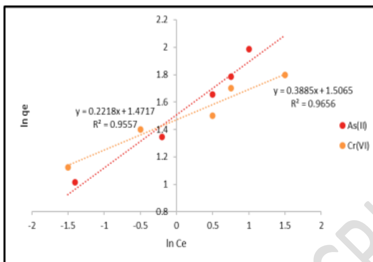
Figure 11 – Freundlich isotherm plot for the adsorption of heavy metals using neem leaf biochar
