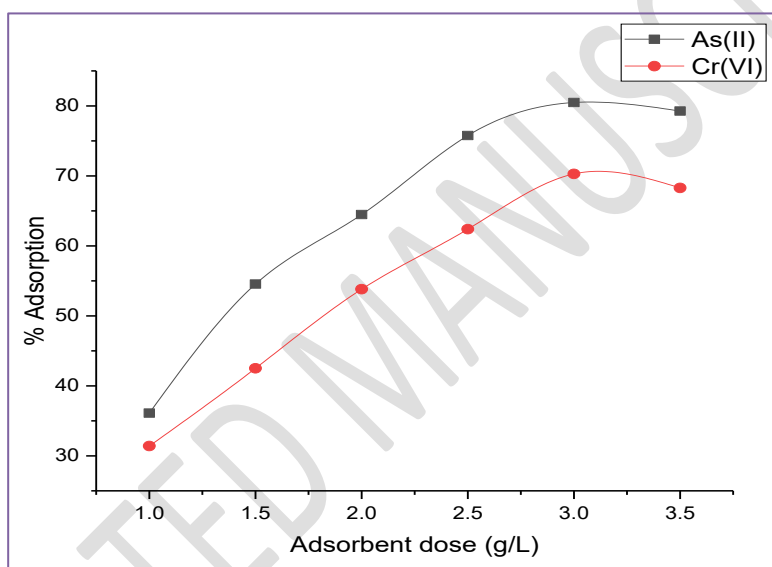
Figure 6 – Changes in adsorption efficiency by varying neem leaf biochar dose
