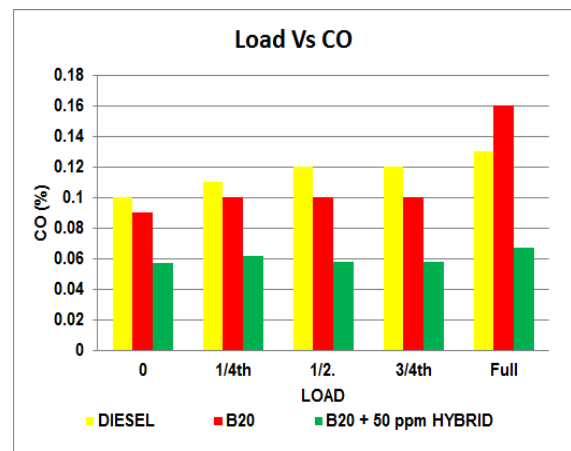
Figure 5. CO Emissions Vs Load
