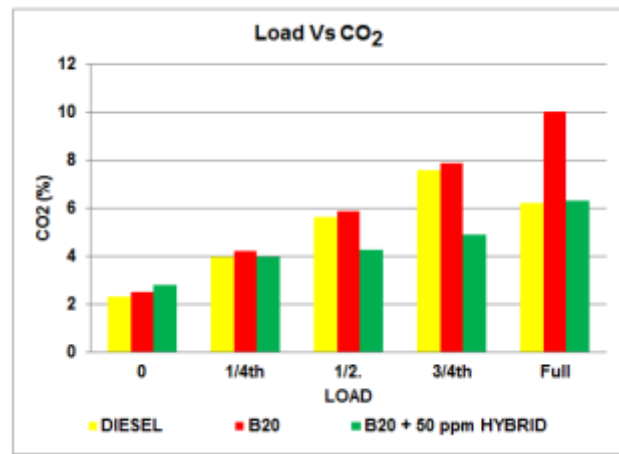
Figure 6: CO 2 Emissions Vs Load
