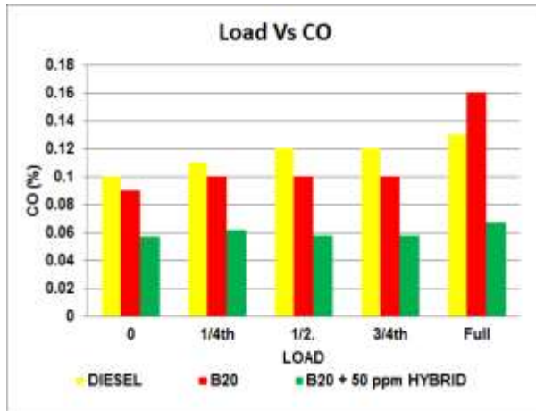
Figure 5: CO Emissions Vs Load
