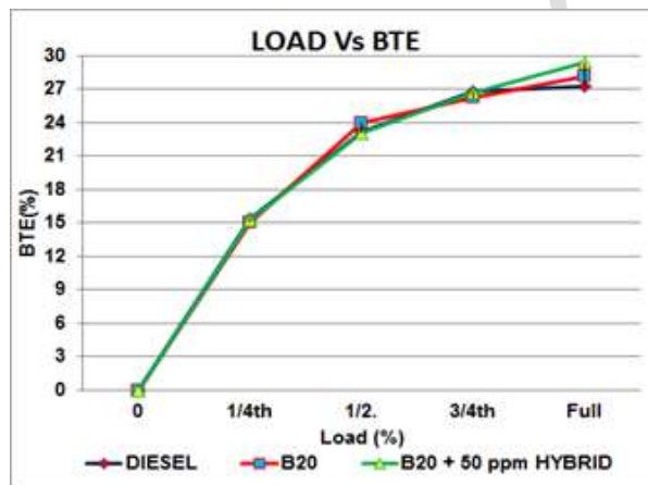
Figure 1: Brake Thermal Efficiency Vs Load
