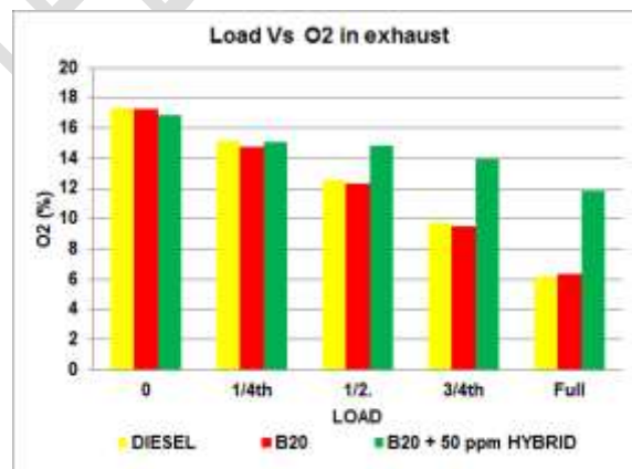
Figure 7: Variation of Excess Oxygen with Load
