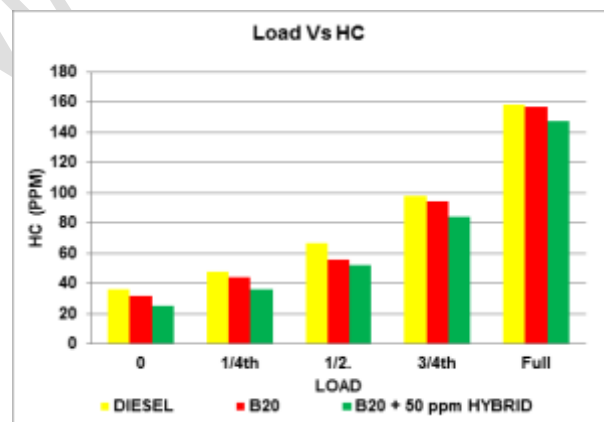
Figure 4: HC Vs Load
