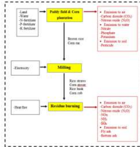
Figure 5. System Boundaries of Existing Treatment Systems: Open Combustion
