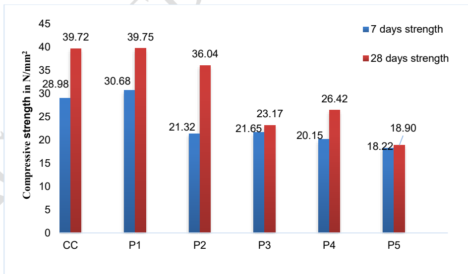
Fig. 4 Compressive strength test
