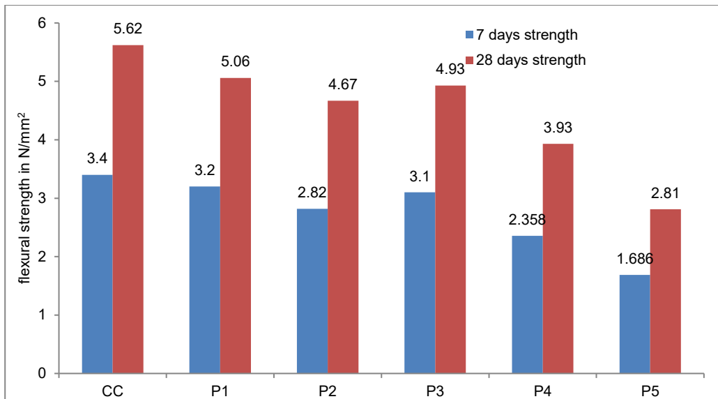
Flexural strength, Figure 6
