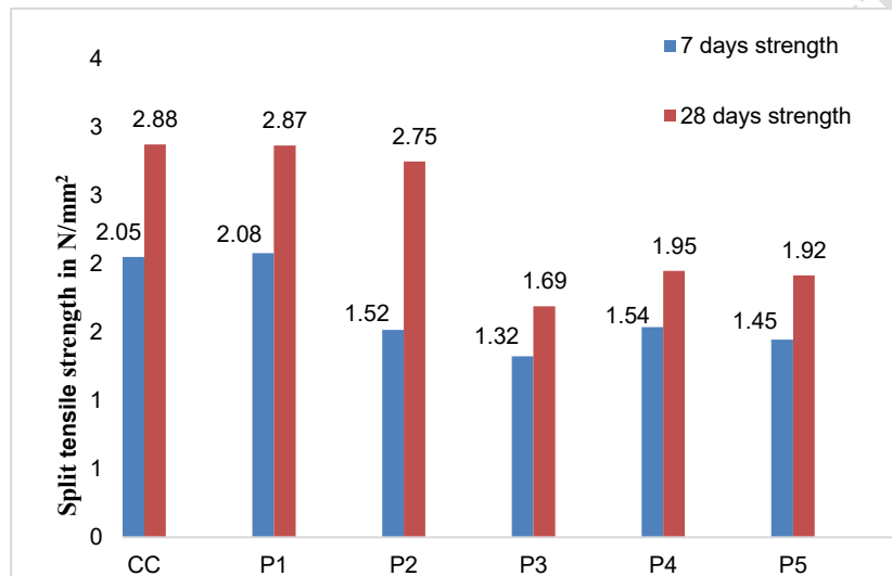
Split tensile strength, Figure 5.
