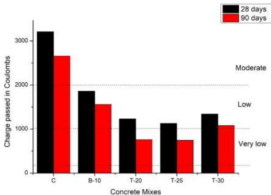
Figure. 8. Total charge passed at 28 and 90 days
