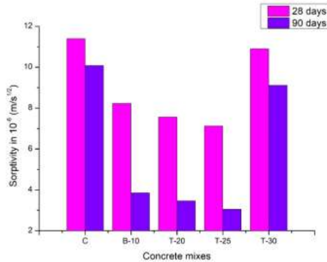
Figure. 9. Sorptivity value at 28 and 90 days
