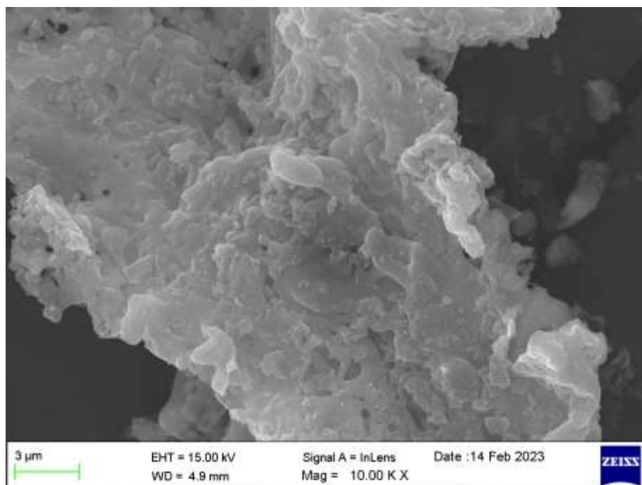
Figure. 1c. SEM Image of SBA
