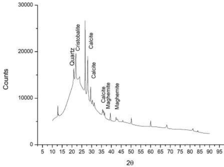
Figure.1b. XRD pattern of SBA
