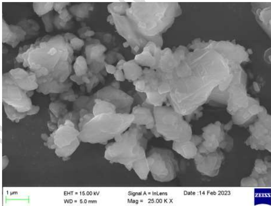
Figs. 2.c. SEM Image of limestone
