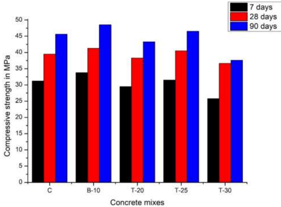
Figure.5. Compressive strength of concrete mixes at 7, 28 and 90 days of curing
