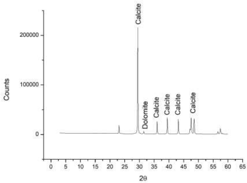
Figure.2b. XRD pattern of limestone
