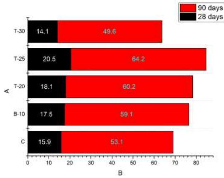
Figure.10. Electrical resistivity at 28 and 90 days
