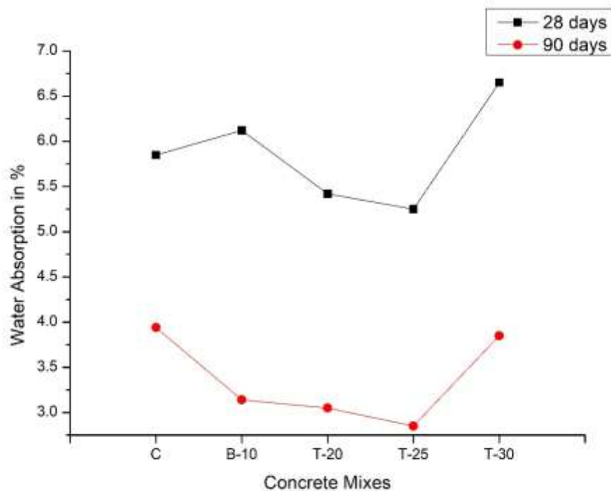
Figure. 6. Water absorption at 28 and 90 days of curing
