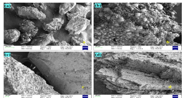
Figure 4. SEM micrograph of the Cupola Slag
