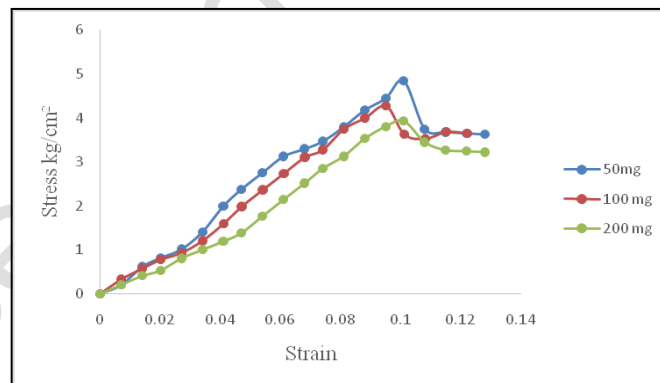
Fig.21: Stress-strain curve of zinc-contaminated soil
