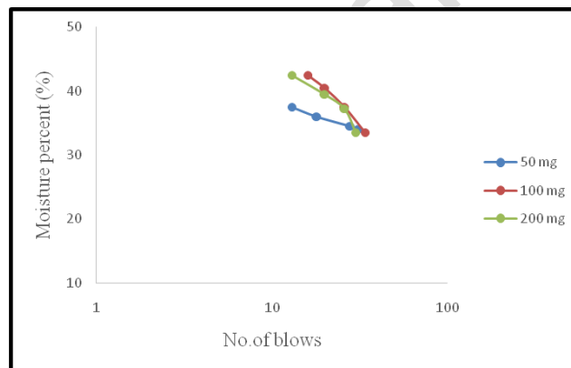
Fig.7: Flow curve of zinc-contaminated soil
