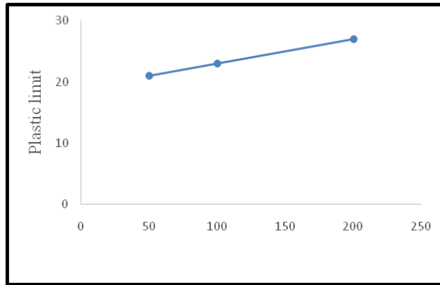
Fig.8: Plastic limit of zinc-contaminated soil
