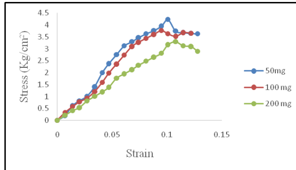
Fig.11: Stress-strain curve of zinc-contaminated soil
