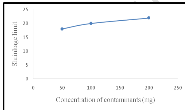
Fig.9: Shrinkage limit of zinc-contaminated soil
