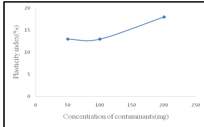
Fig.15: Plasticity index of zinc-contaminated soil
