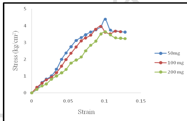
Fig.16: Stress-strain curve of zinc-contaminated soil
