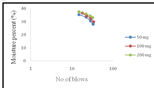
Fig.12: Flow curve of zinc-contaminated soil
