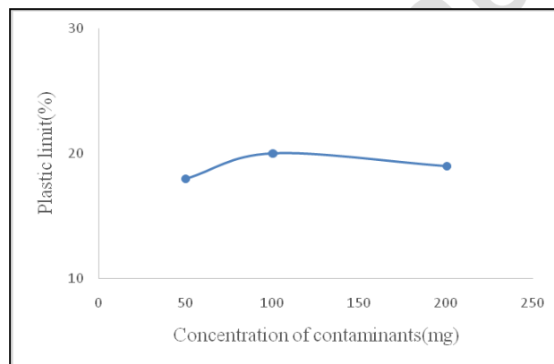
Fig.18: Plastic limit of zinc-contaminated soil
