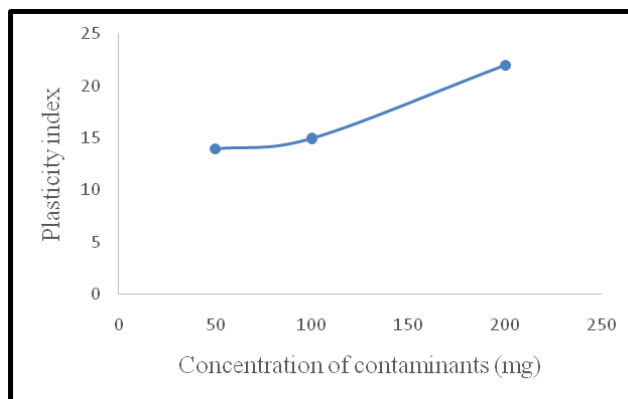
Fig.10: Plasticity index of zinc-contaminated soil
