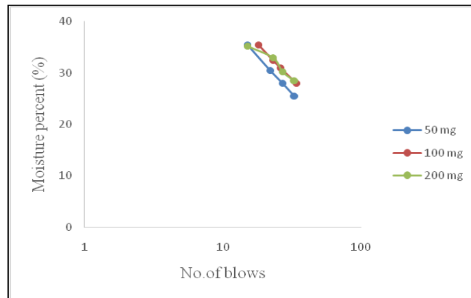
Fig.17: Flow curve of zinc-contaminated soil
