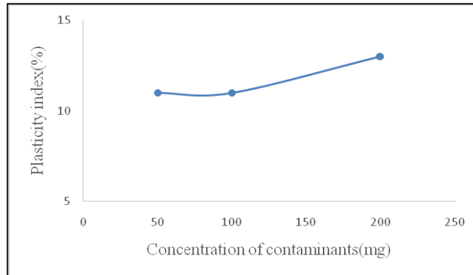
Fig.20: Plasticity Index of zinc-contaminated soil
