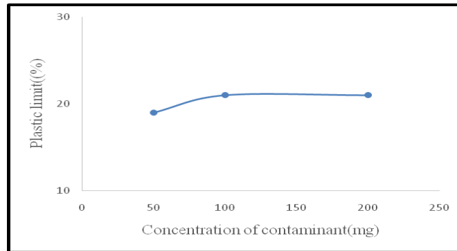
Fig.13: Plastic limit of zinc-contaminated soil
