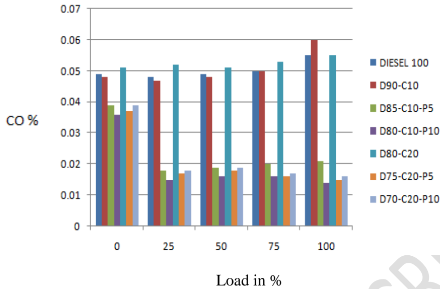
Figure 5 CO Vs Load
