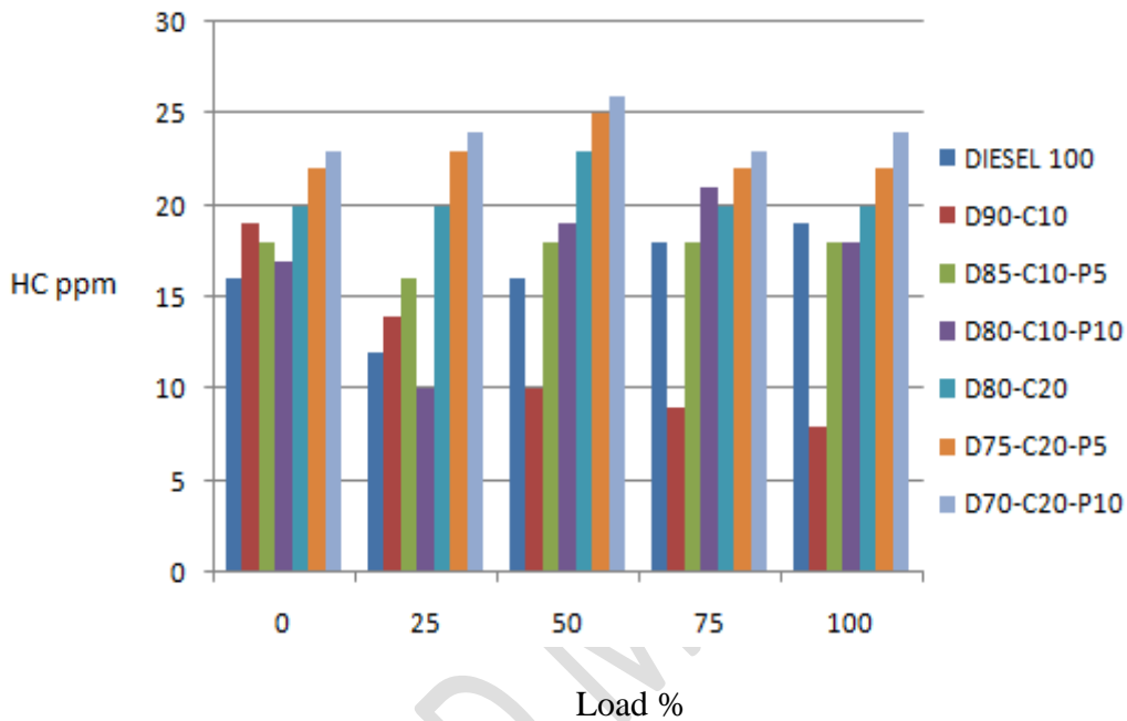
Figure 8 HC Vs Load
