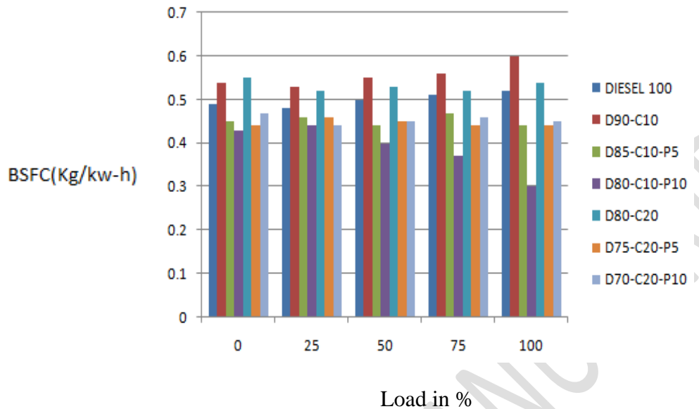
Figure 4 BSFC Vs Load
