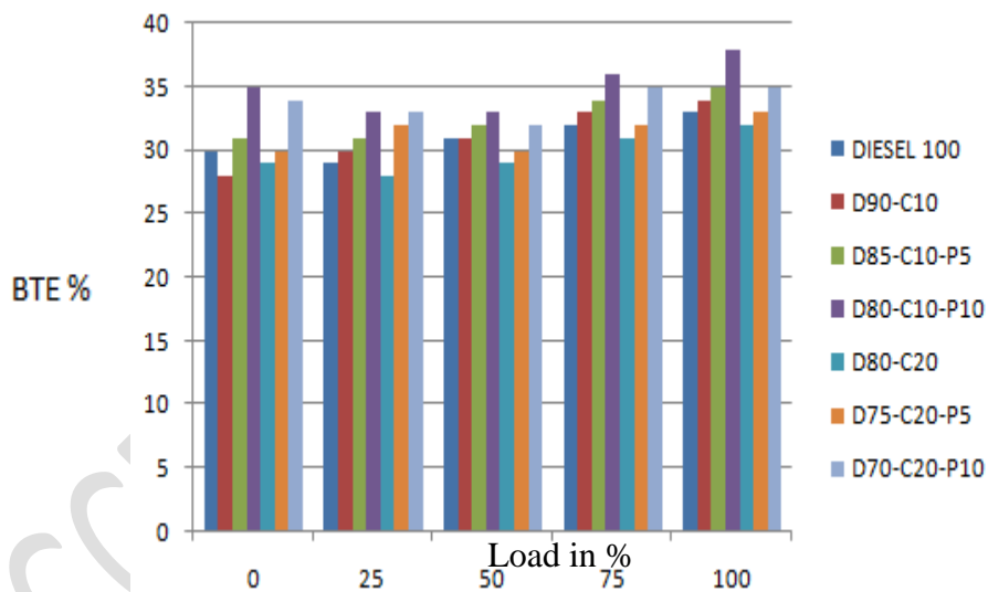
Figure 3 BTE Vs Load
