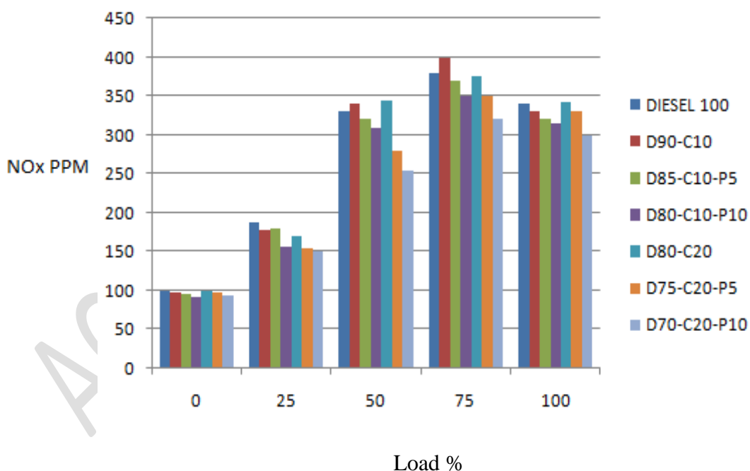
Figure 7 NO x Vs Load
