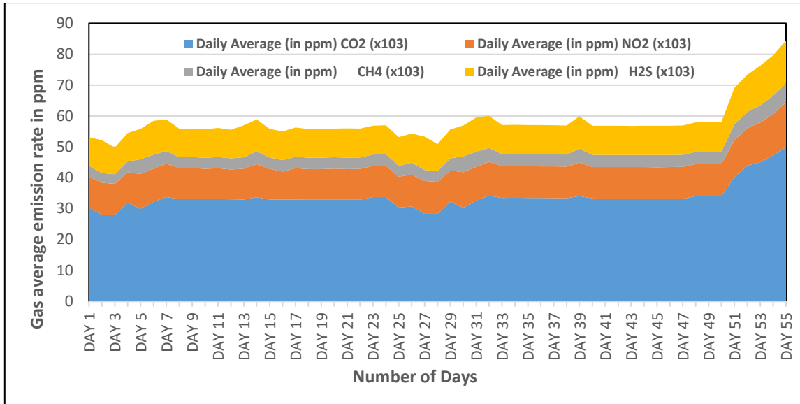
Figure 8. Graphical representation of various gas emission rate statistics
