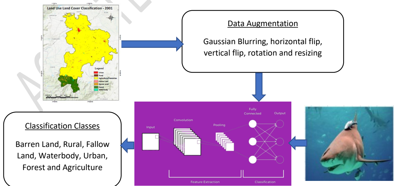
Figure 1: Proposed Architecture
