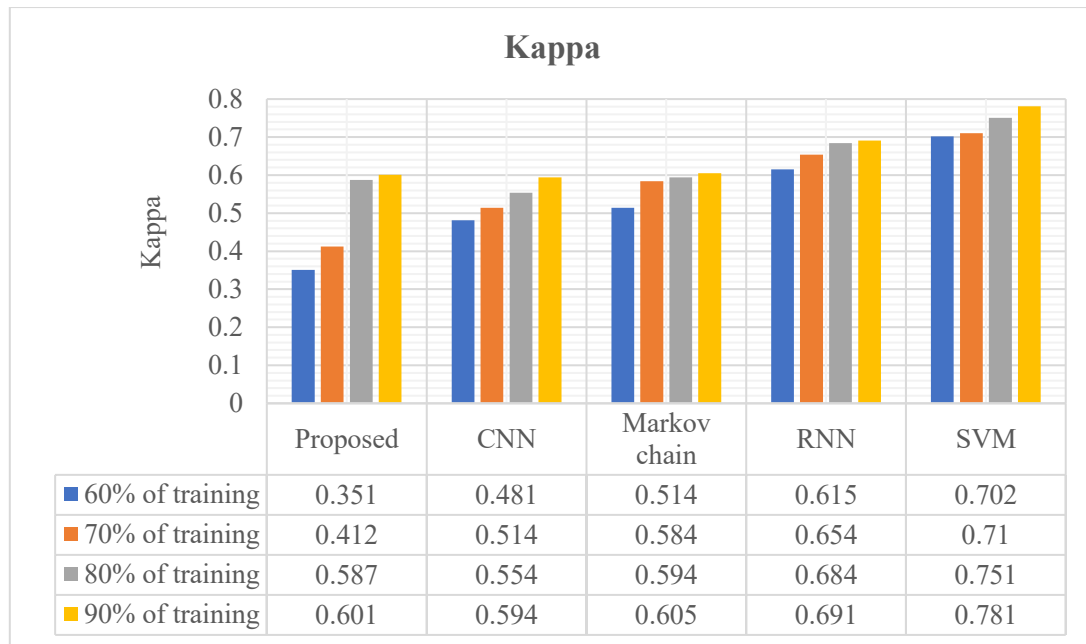
Figure 8: kappa
