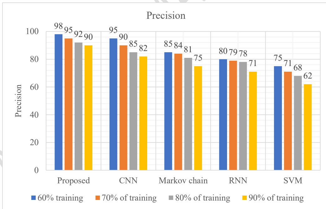
Figure 4: Precision
