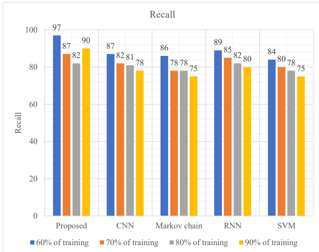
Figure 5: Recall
