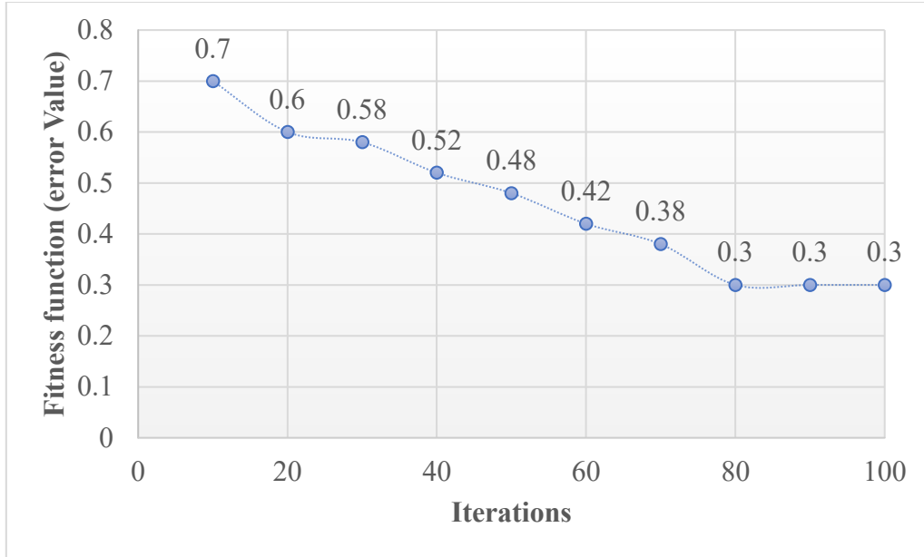
Figure 11: convergence analysis
