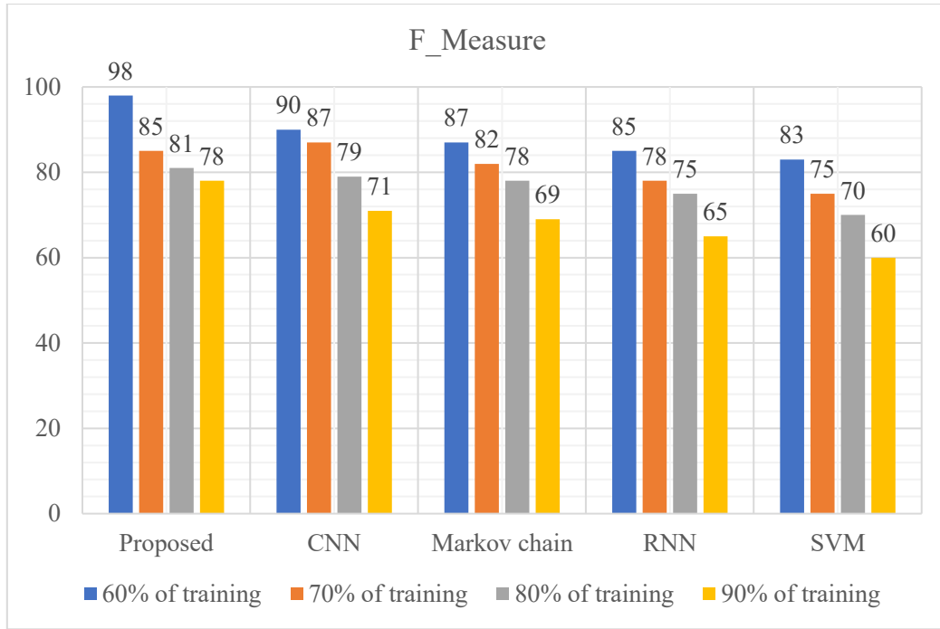
Figure 6: F_Measure
