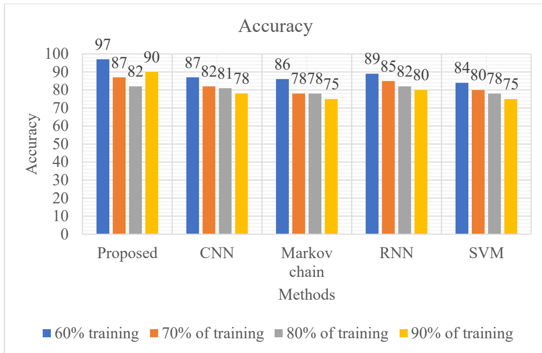
Figure 9: Accuracy
