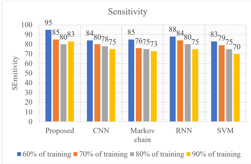
Figure 10: Sensitivity
