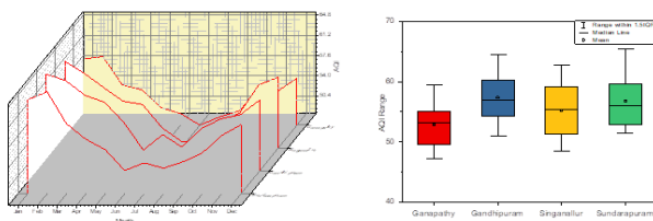
Figure 8. Range of AQI from Jan to Dec 2021
