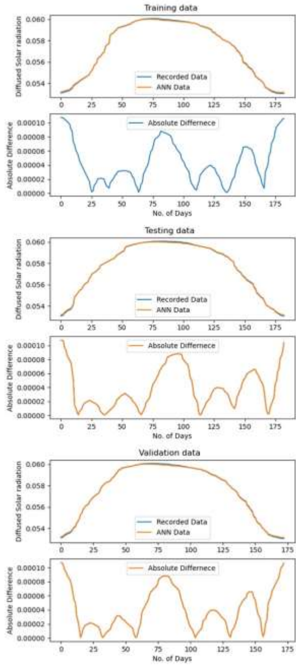
Fig. 4. ANN modeling of Diffused solar radiation for Multan
