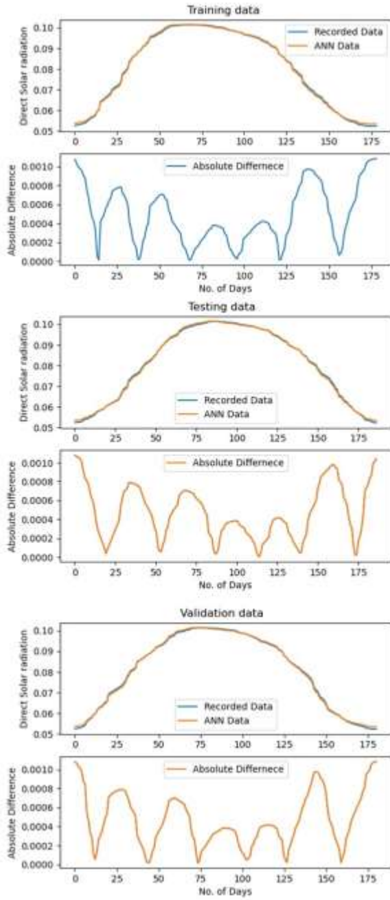
Fig. 7. ANN modeling of Direct beam solar radiation for Multan
