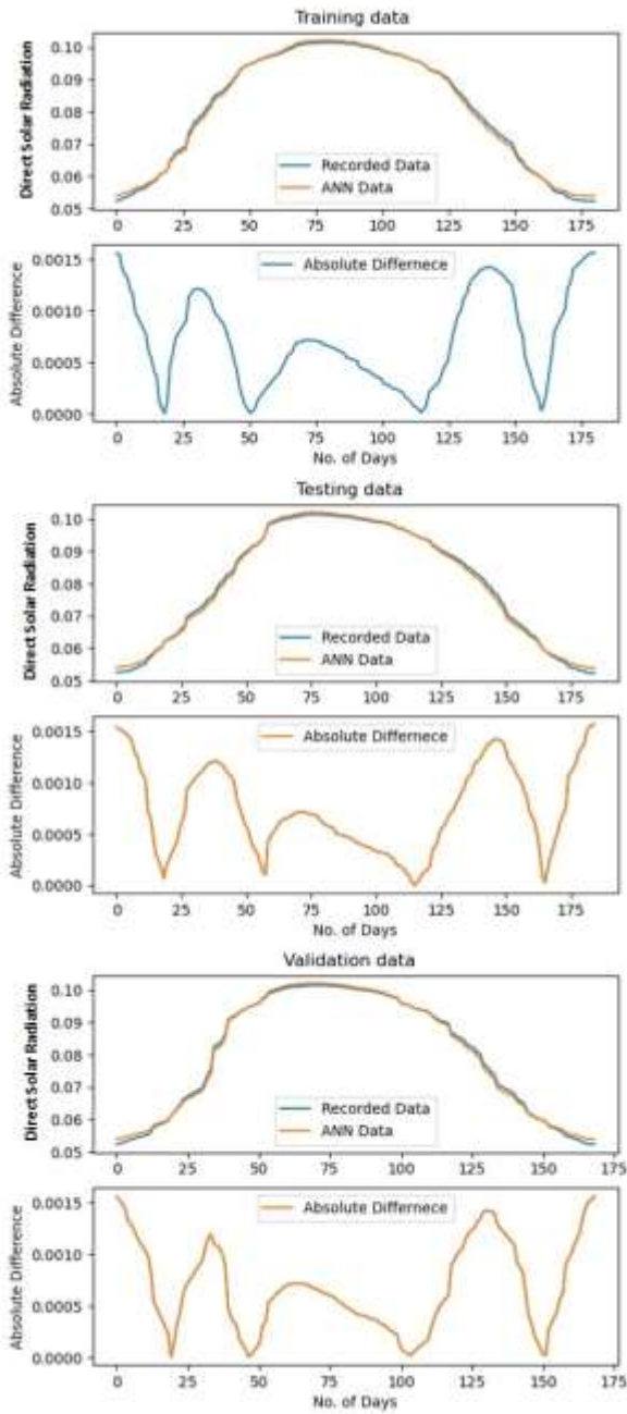
Fig. 13. ANN modeling of Direct beam solar radiation for Multan, using three inputs of solar radiation of Karachi, Lahore, and Quetta
