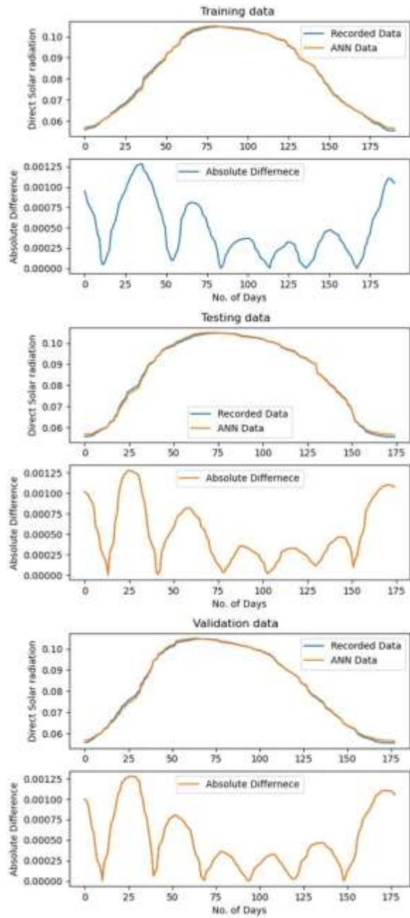
Fig. 8. ANN modeling of Direct beam solar radiation for Quetta
