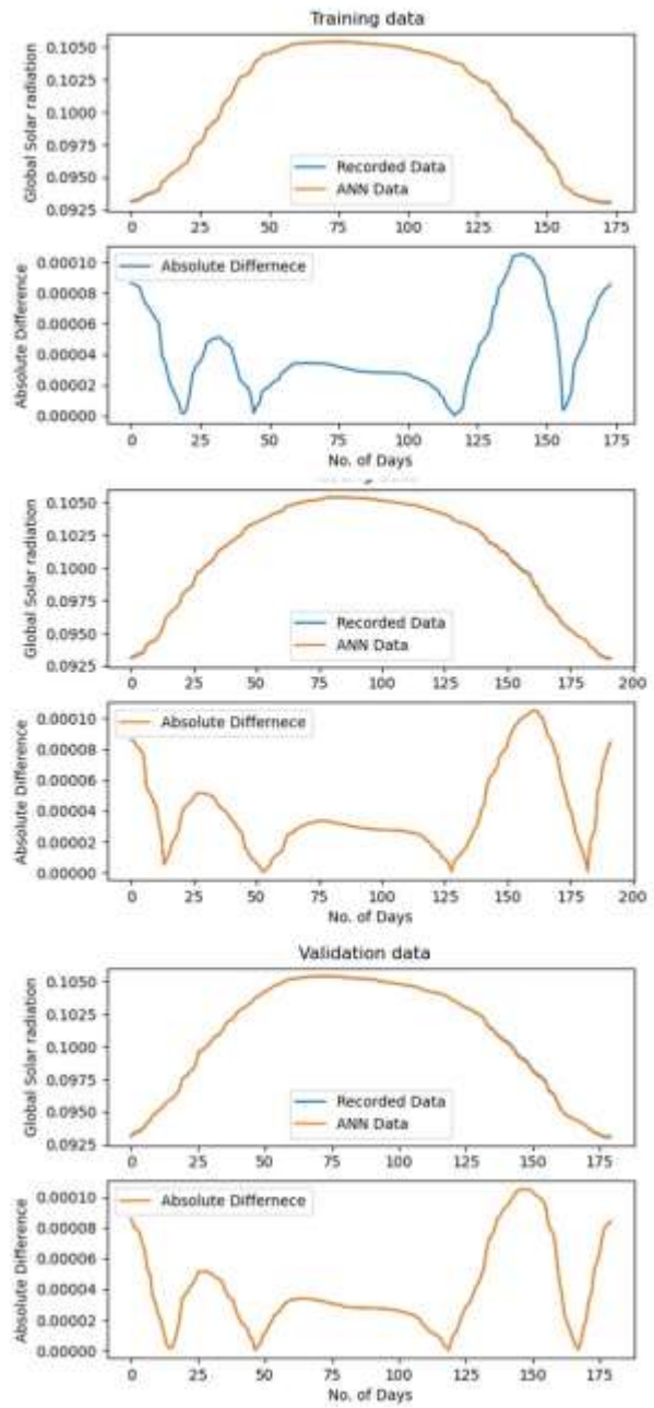
Fig. 14. ANN modeling of Global solar radiation for Multan, using three inputs of solar radiation of Karachi, Lahore, and Quetta
