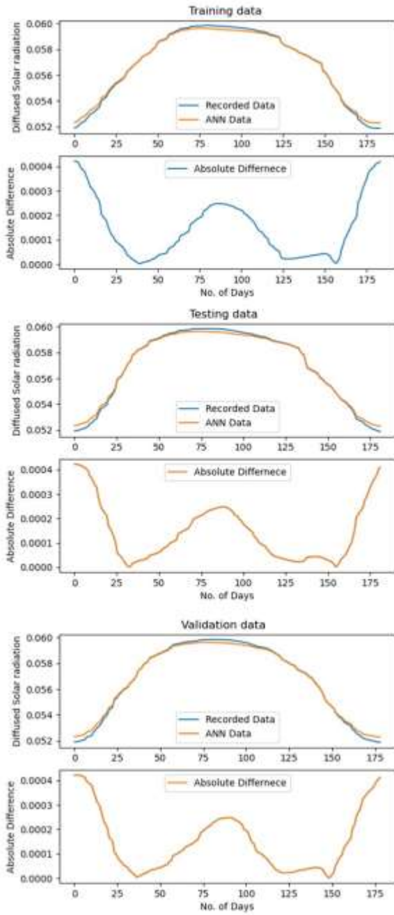
Fig. 3. ANN modeling of Diffused solar radiation for Lahore
