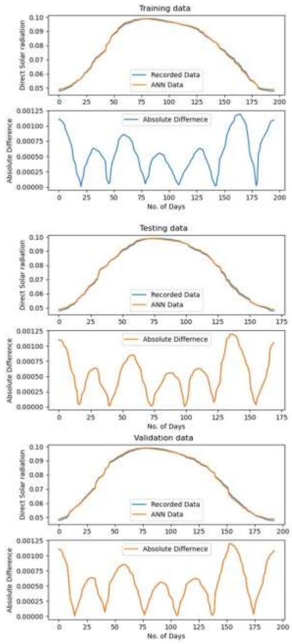
Fig. 6. ANN modeling of Direct beam solar radiation for Lahore
