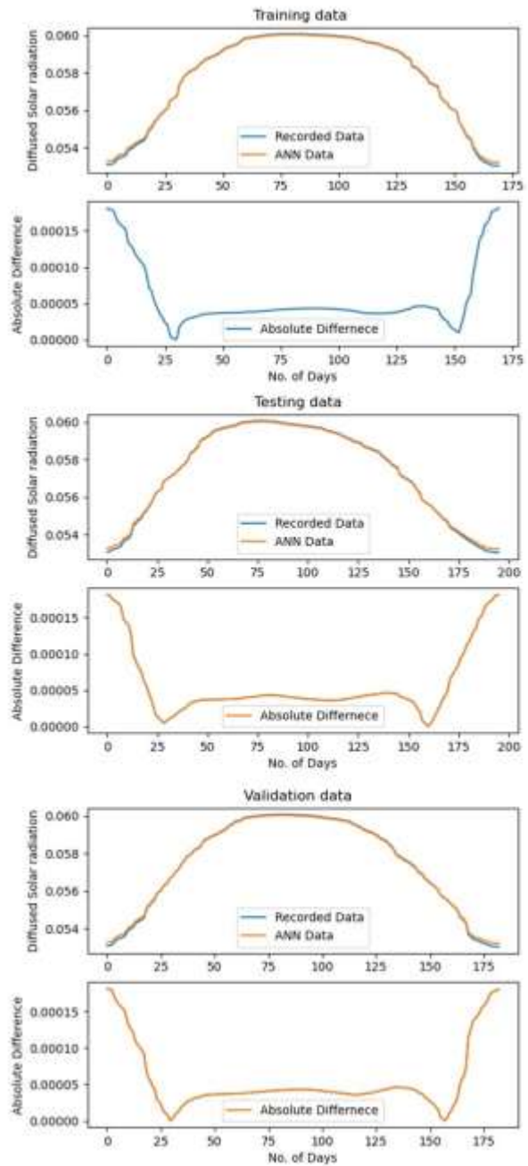
Fig. 12. ANN modeling of Diffused solar radiation for Multan, using three inputs of solar radiation of Karachi, Lahore, and Quetta
