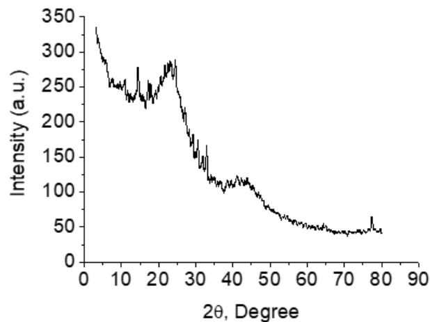
Figure 2. The X-ray diffraction of rice husk activated with CaCl 2 .
