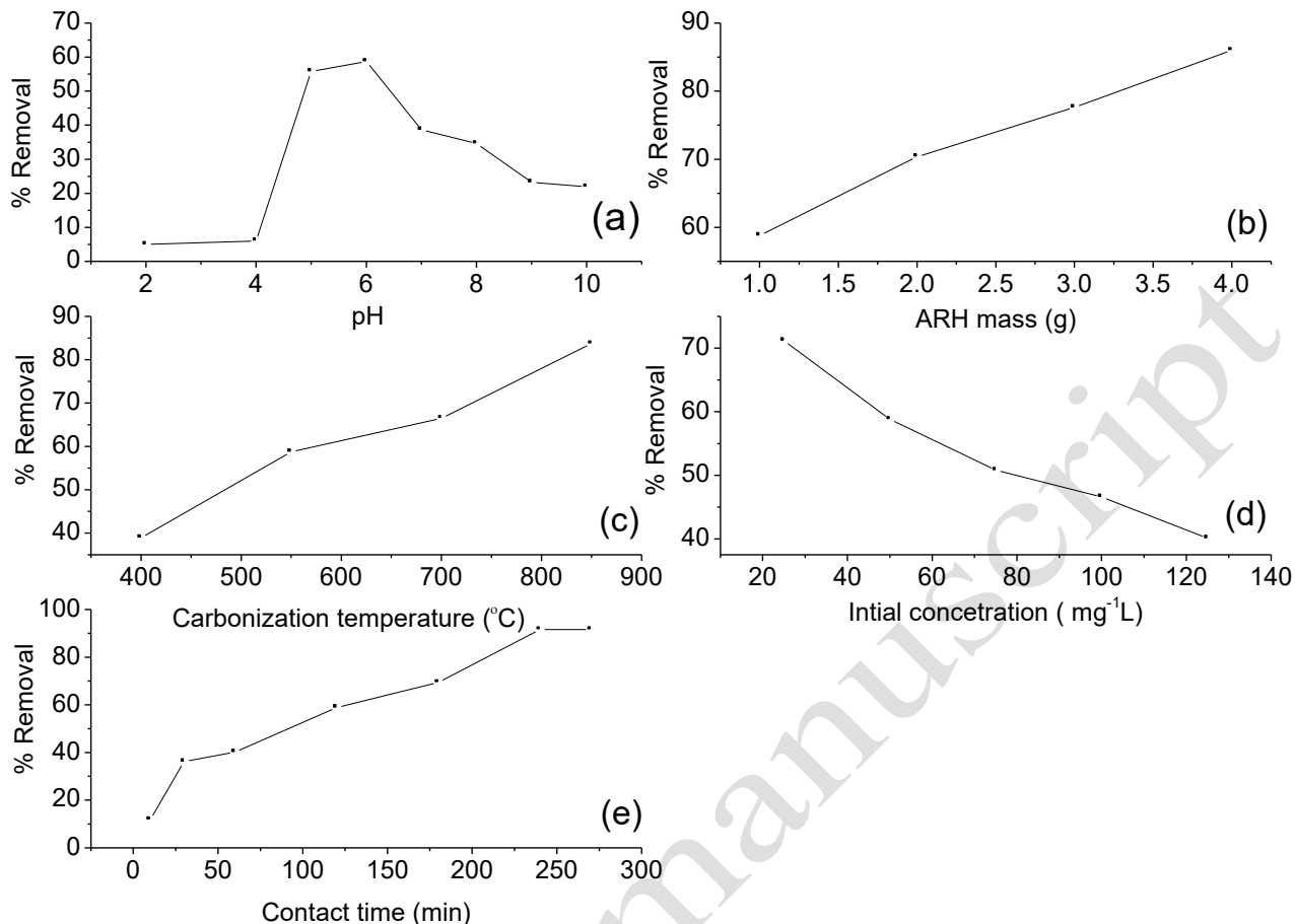
Figure 3. The effect of experimental condition on percent removal of phenol including: effect of (a) pH, (b) ARH mass, (c) carbonization temperature, (d) initial concentration, and (e) contact time.
