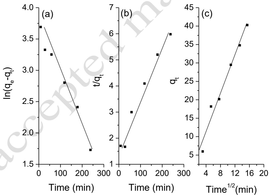
Figure 5: (a) Pseudo first order (b) Pseudo second order, and (c) Intraparticle kinetics models for the adsorption of phenol on ARH at pH=6, the carbonization temperature= 550 °C, the contact time = 2hrs, ARH mass=1 g/ 1L, and phenol concentration range= 25-125
