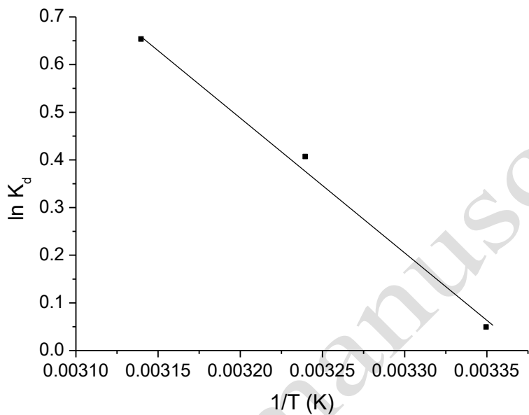
Figure 6. Van't Hoff plot for the adsorption of phenol on ARH at pH=6, Temperature = (298-318 K), the carbonization temperature= 550 °C, the contact time = 24hrs, ARH mass=1 g/ 1L, and phenol concentration range= 25-125 mg -1 L
