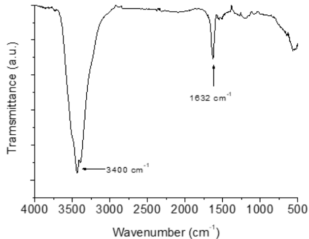
Figure 1. FTIR spectrum of rice husk activated with CaCl 2 .
