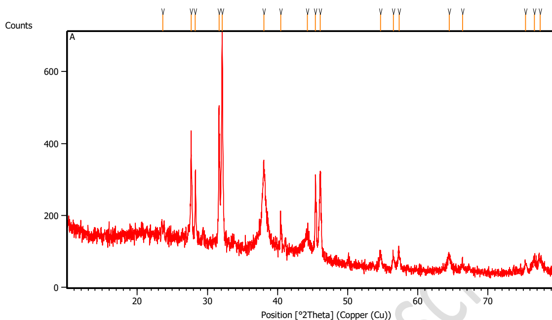
Figure 5 – Graph showing XRD analysis
