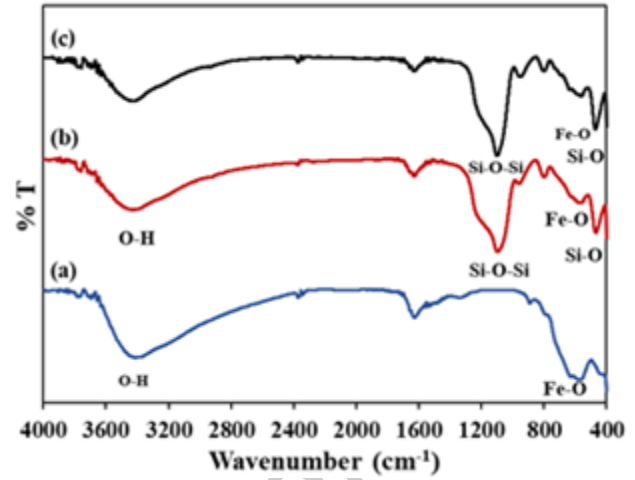
Figure 2. FTIR spectra of (a) \text{Fe}_3\text{O}_4 , (b) \text{Fe}_3\text{O}_4/\text{SiO}_2 , and (c) \text{Fe}_3\text{O}_4/\text{SiO}_2/\text{NiO}
