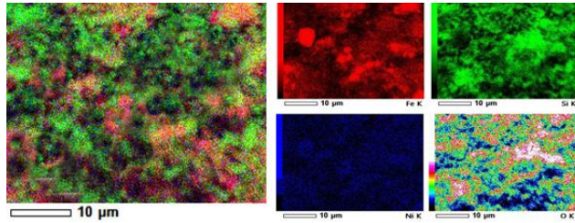
Figure 5. SEM Mapping of \text{Fe}_3\text{O}_4/\text{SiO}_2/\text{NiO}
