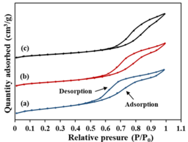
Figure 3. \text{N}_2 adsorption-desorption isotherm of (a) \text{Fe}_3\text{O}_4 , (b) \text{Fe}_3\text{O}_4/\text{SiO}_2 , and (c) \text{Fe}_3\text{O}_4/\text{SiO}_2/\text{NiO}
